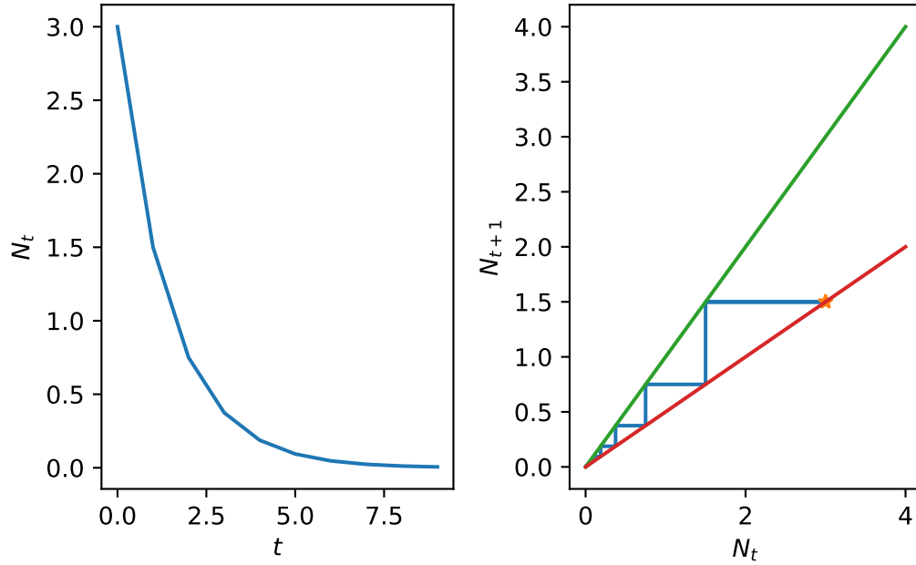
Figure 2.5: A cobweb plot of the Malthusian model solution when r=0.5 . (a) Time series and (b) Cobweb diagrams.
