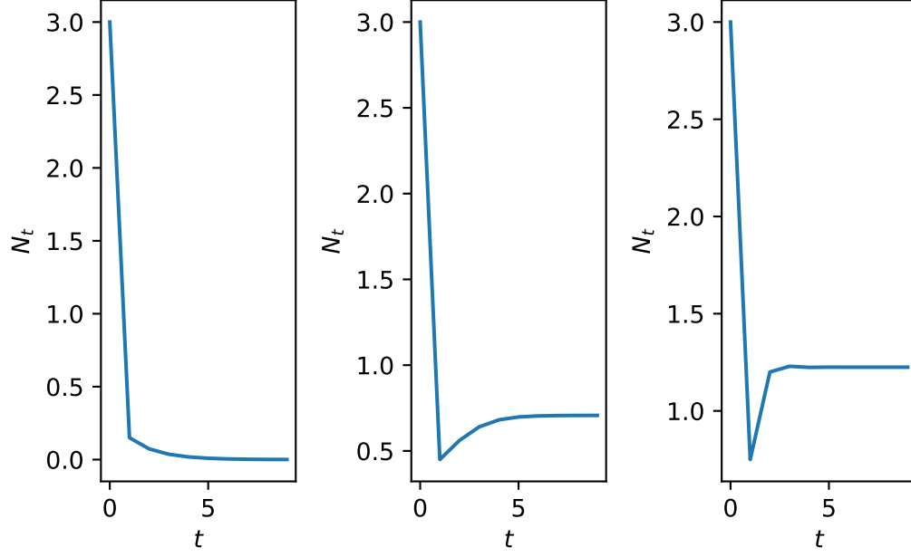
Figure 2.6: Time series solution for (a) \gamma=0.5 and (b) \gamma=1.5 and (c) \gamma=10.5 .
