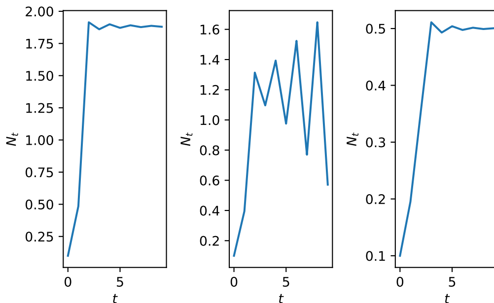
Figure 2.10: Time series solution for different values of h .
