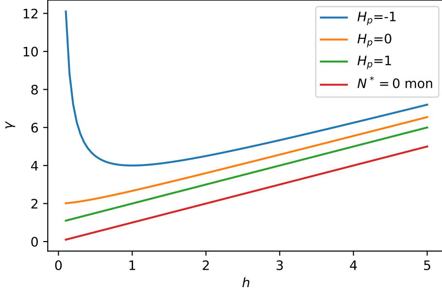
Figure 2.12: Stability regions for the harvesting model.
