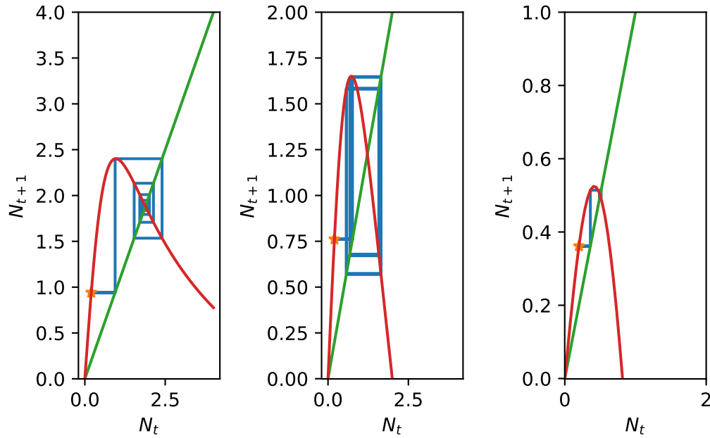
Figure 2.13: Cobweb diagrams for different values of h .
