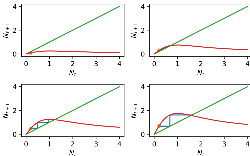
Figure 2.8: Cobweb diagrams for different values of \gamma .
