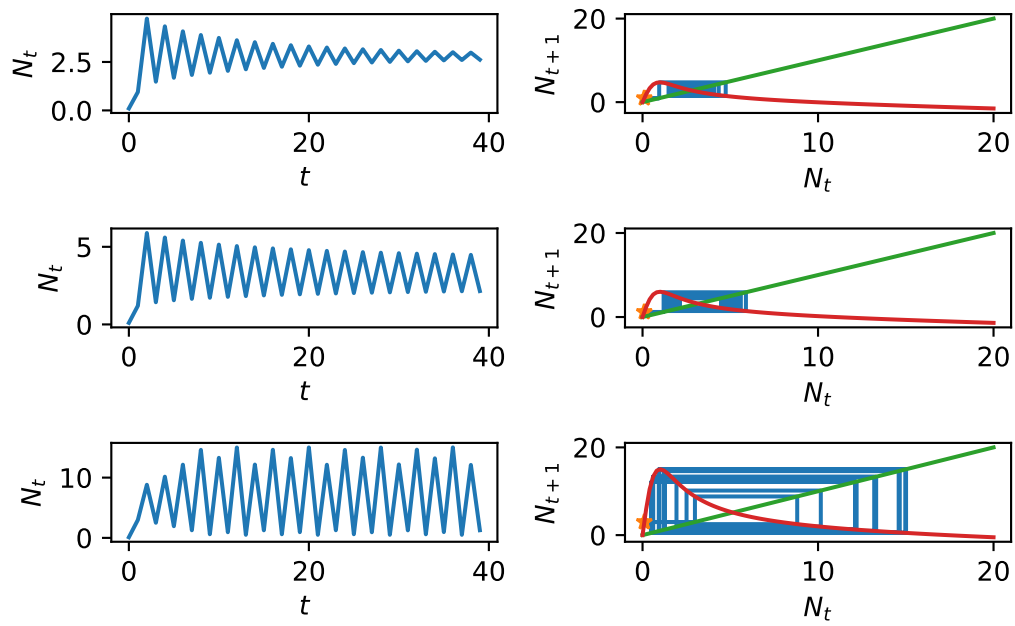
Figure 2.14: Transition from period 2 to period 4 solutions in the harvesting model
