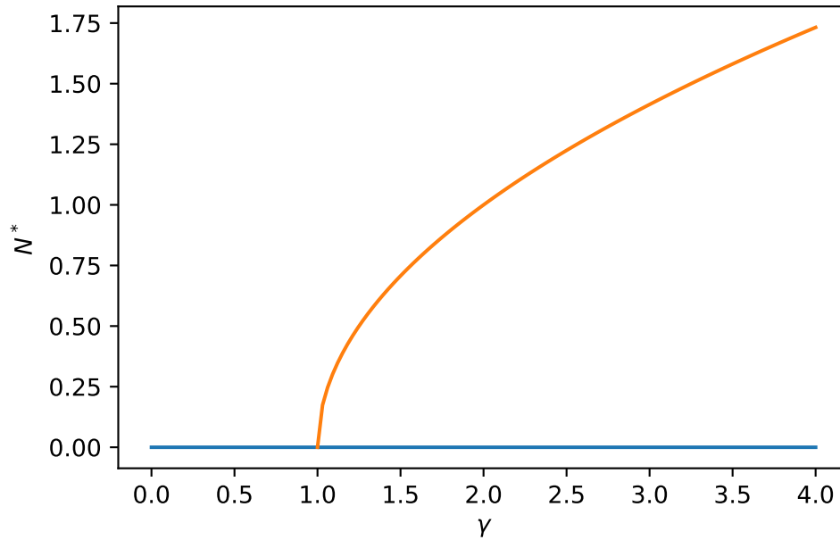
Figure 2.9: A bifurcation diagram.
