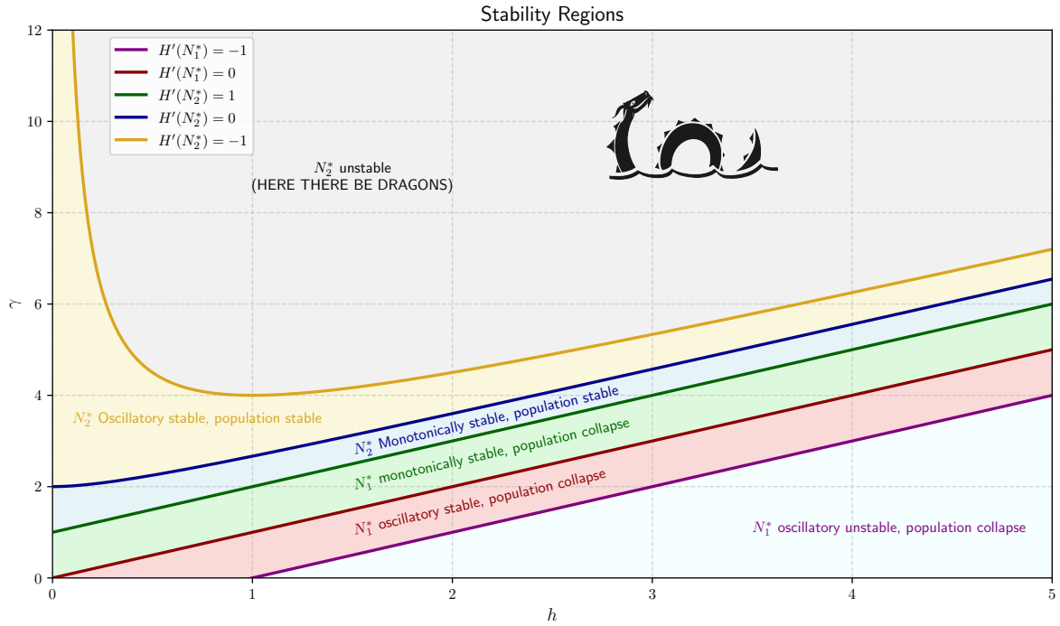
Figure 2.15: Stability regions from studying the linear stability of the fixed points of the harvesting model. This is not enough to understand population stability/collapse for the grey region, as can be seen in Figure 2.16
