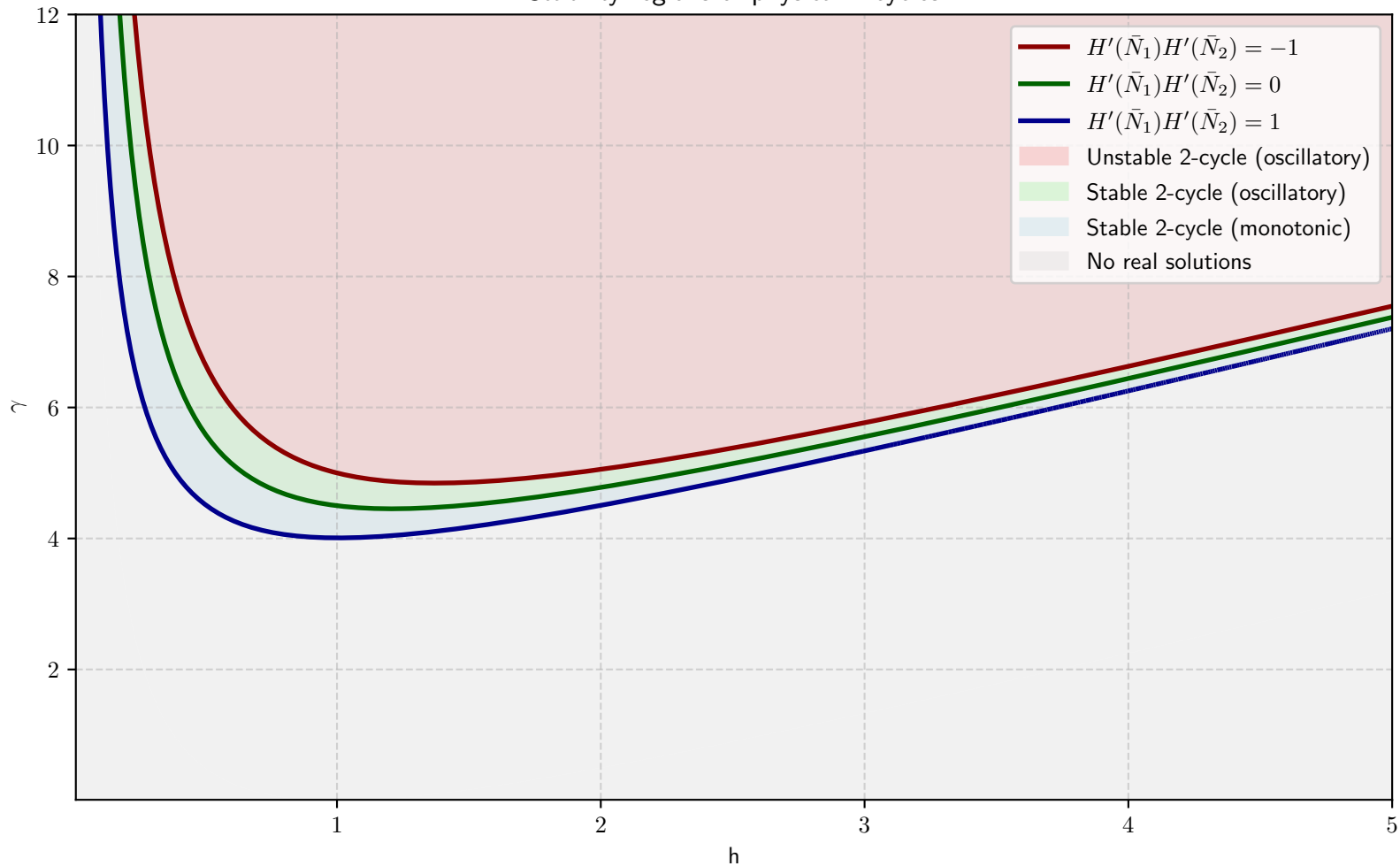
Stability regions of physical 2-cycles
