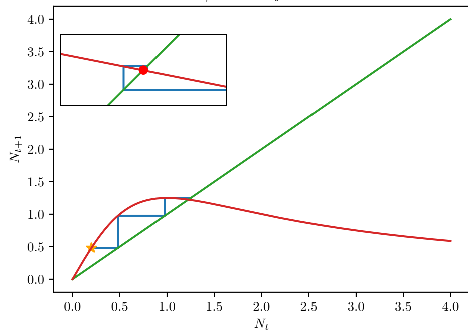
\gamma = 2.5, N_0 = 0.2
