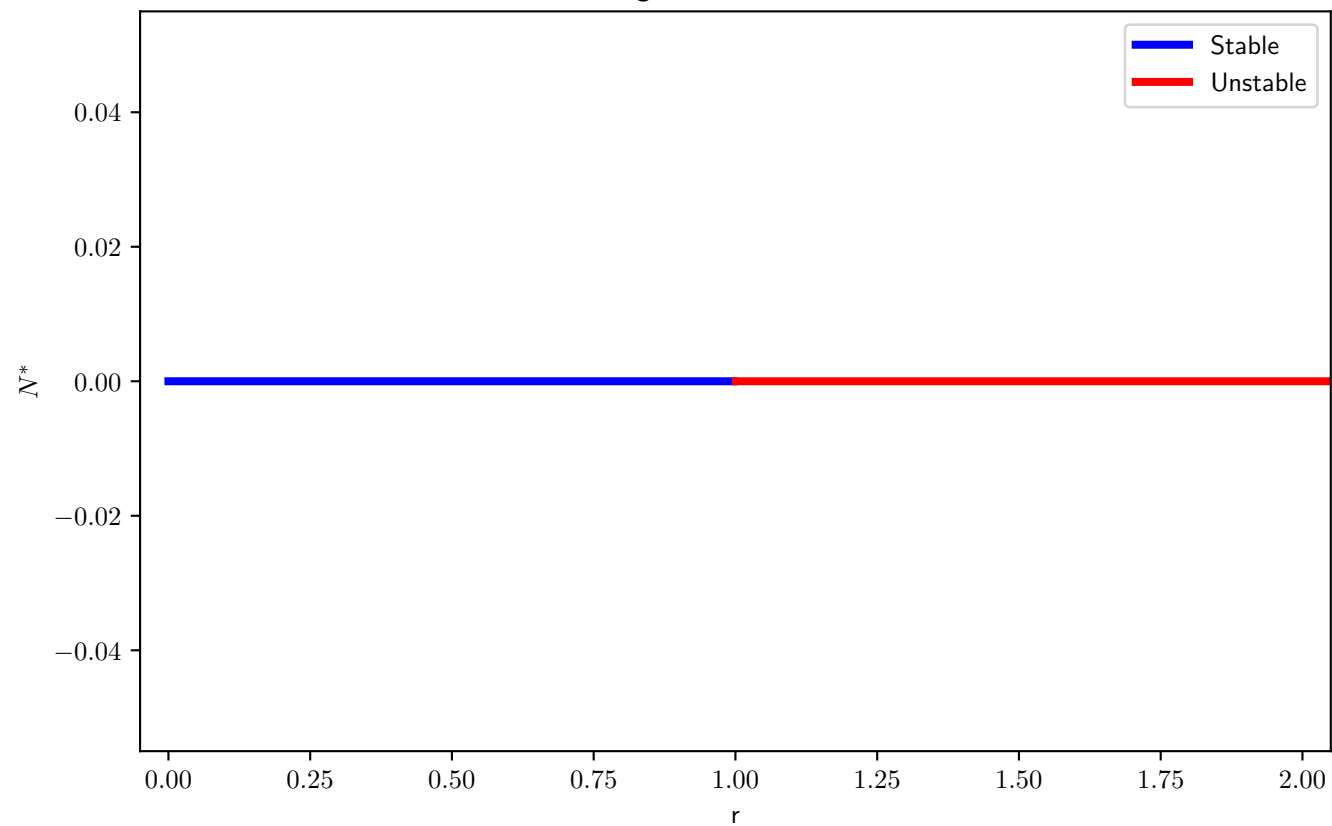
Bifurcation Diagram of the Malthusian Model
