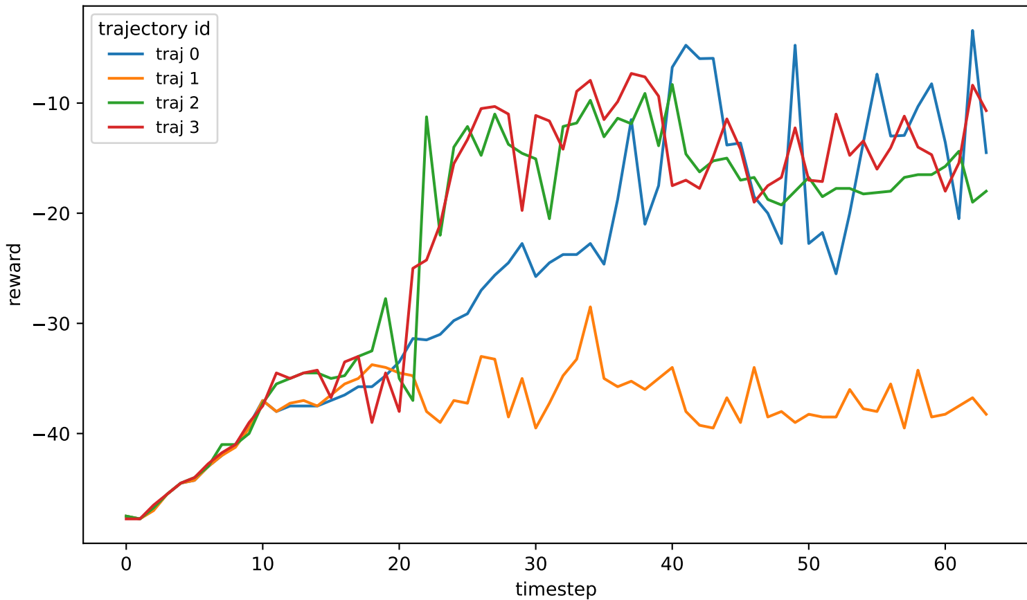
Task 1 trajectories 1
