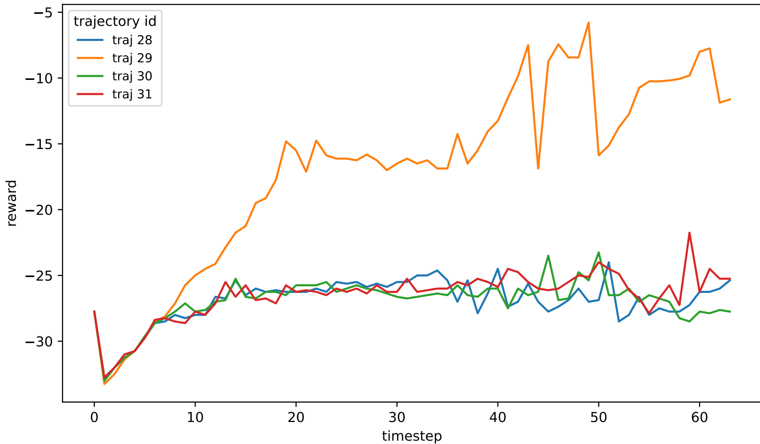
Task 3 trajectories 1
