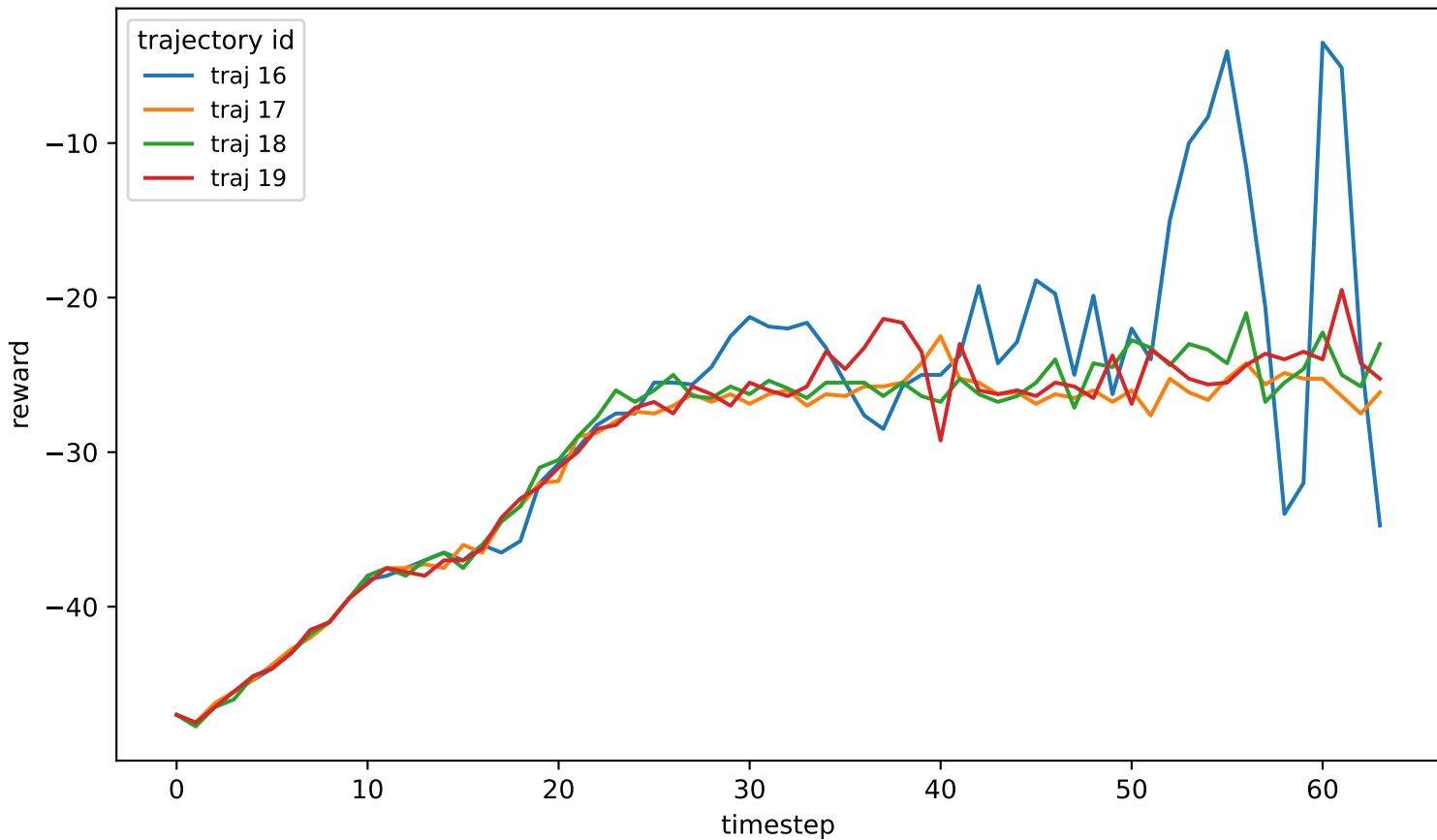
Task 1 trajectories 2
