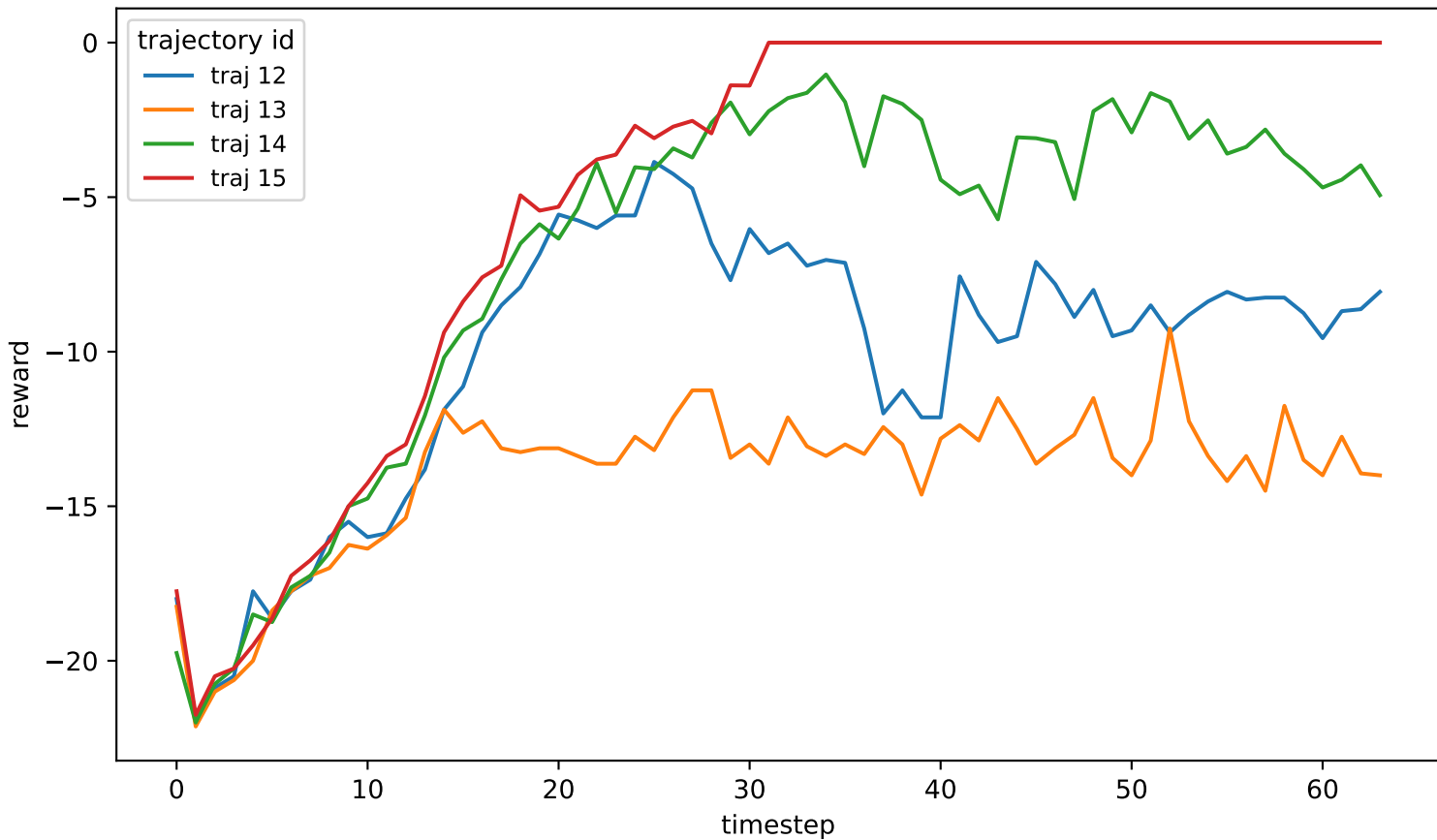
Task 0 trajectories 1
