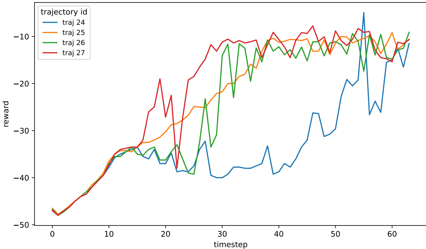
Task 1 trajectories 3
