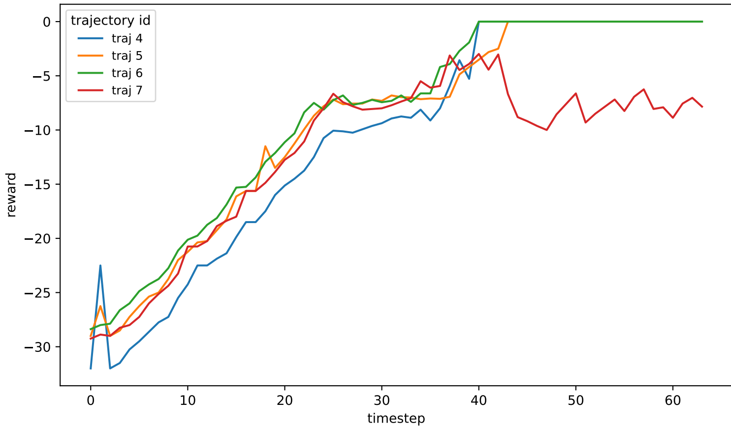
Task 7 trajectories 1
