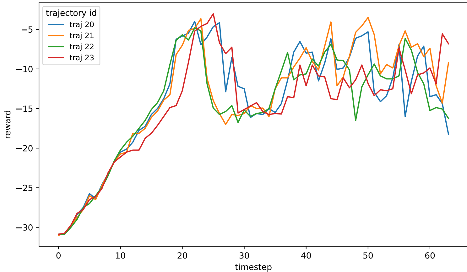
Task 9 trajectories 1
