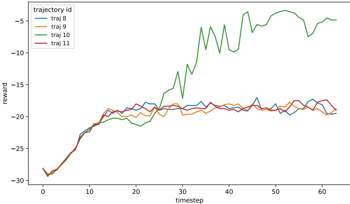
Task 6 trajectories 1
