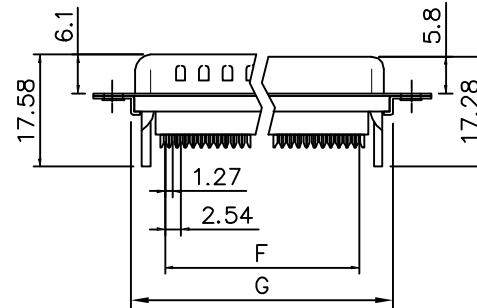
Without Insulator Support
