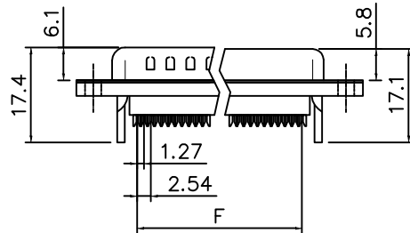
With Insulator Support
