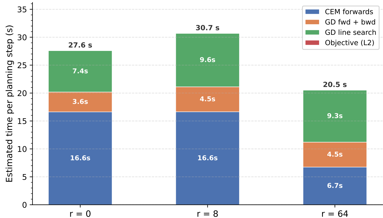
CEM-GD Planning Step Time Breakdown (CEM: 10 iter \times 100 samples \times H=6 | GD: 10 steps \times 8 line-search)
