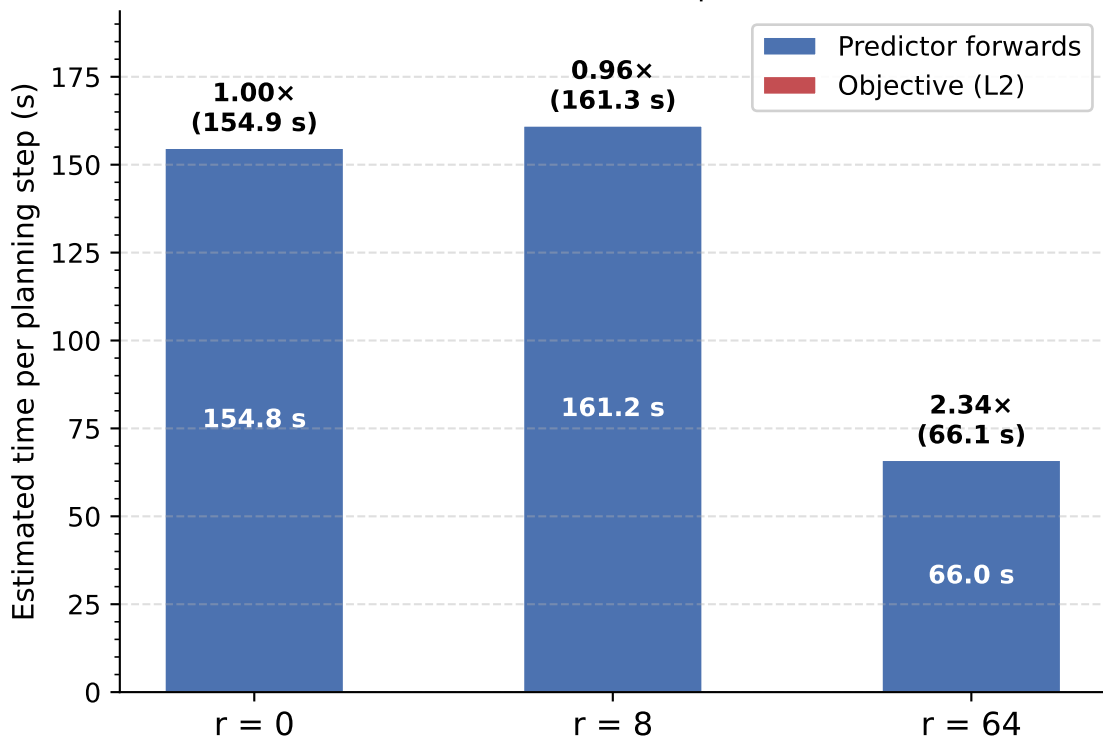
CEM Planning Step Time Breakdown (30 iterations \times 300 samples \times H = 6)
