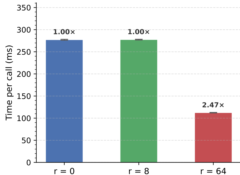
CEM forward (B = 100)
