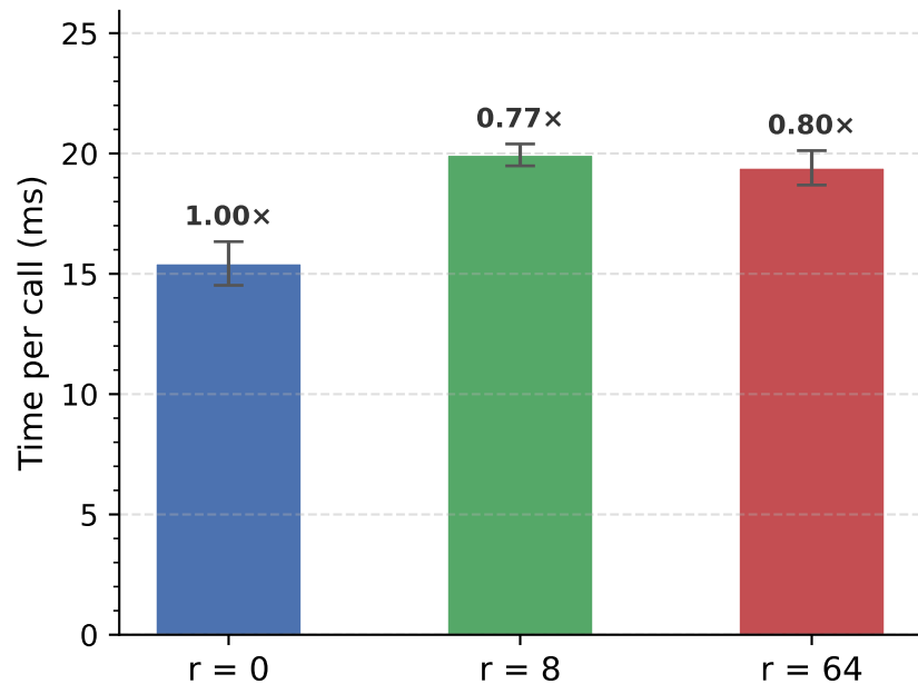
GD line-search forward (B = 1)
