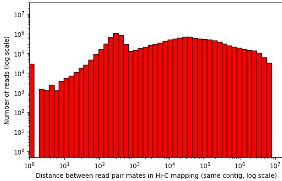
Mate distance distribution for first 20000001 read pairs for sample SRR8238190.on.FI1.samblaster.bam
