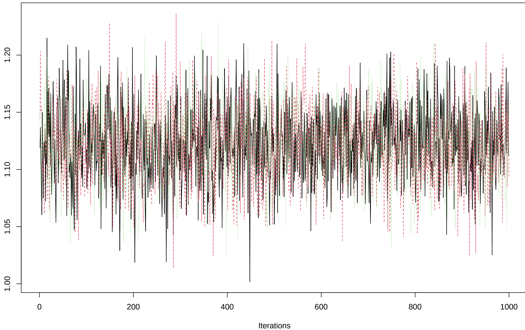
Trace of summer
