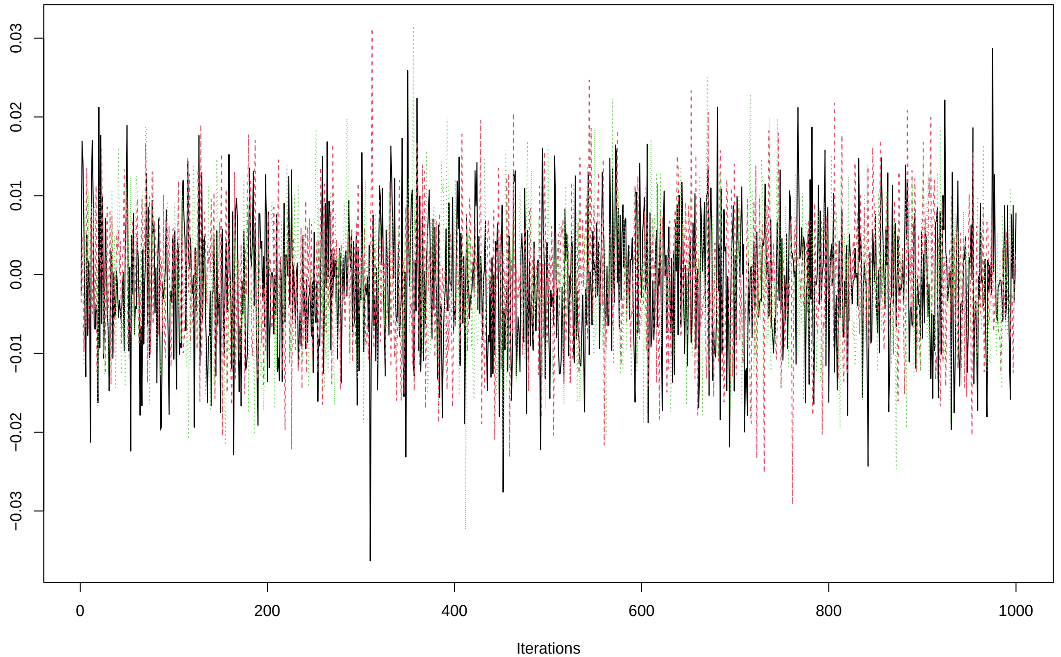
Trace of pptconc
