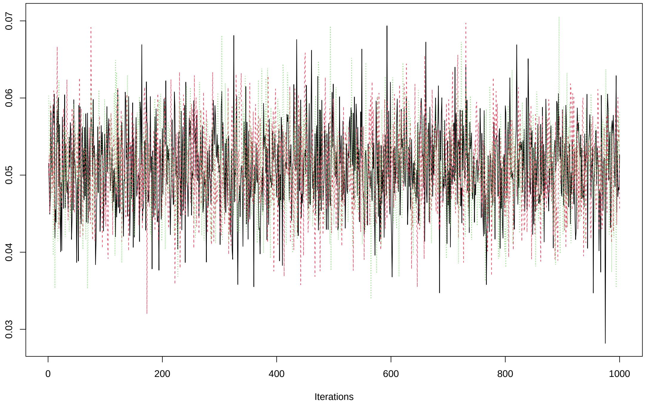
Trace of PATot
