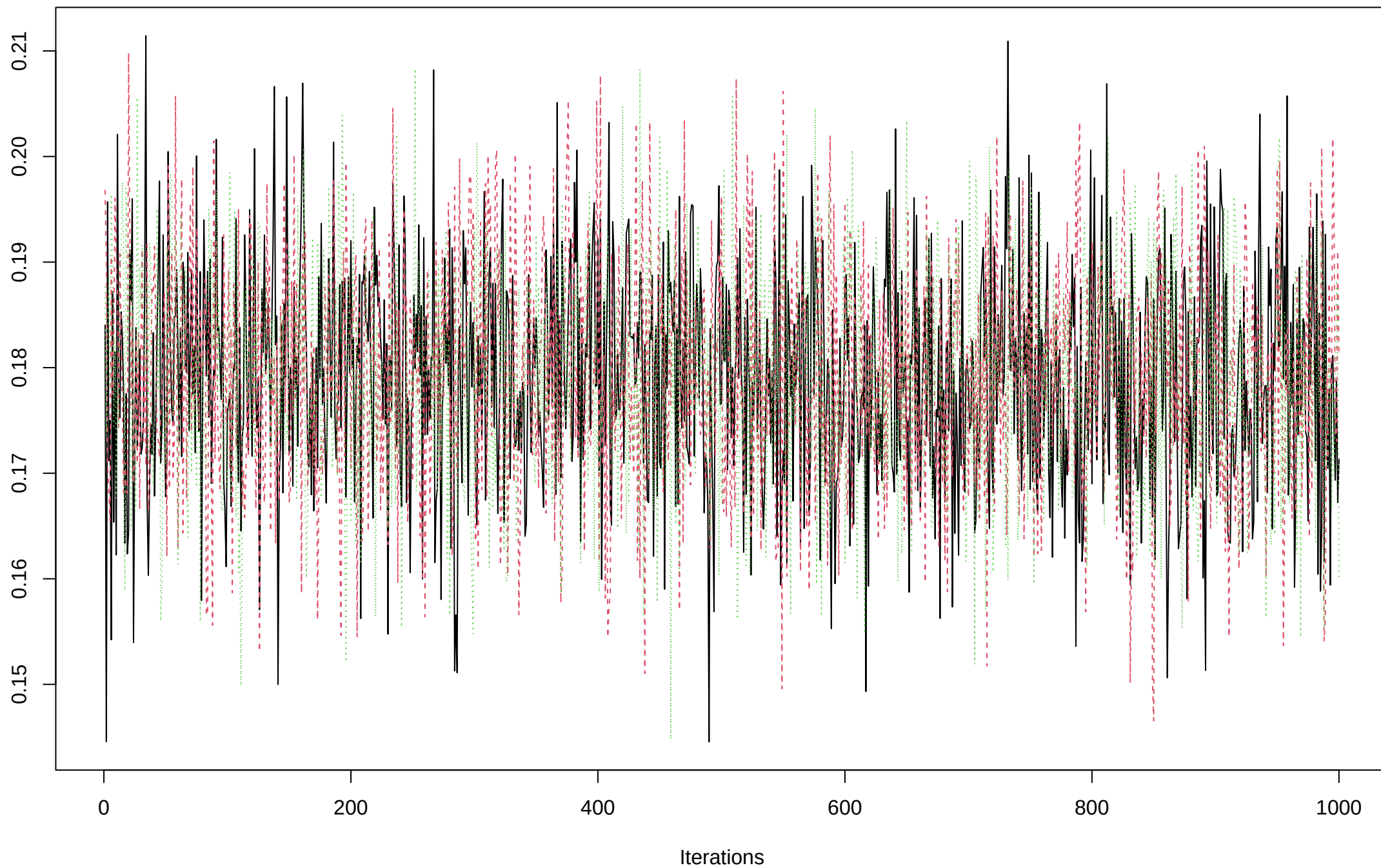
Trace of TSAve
