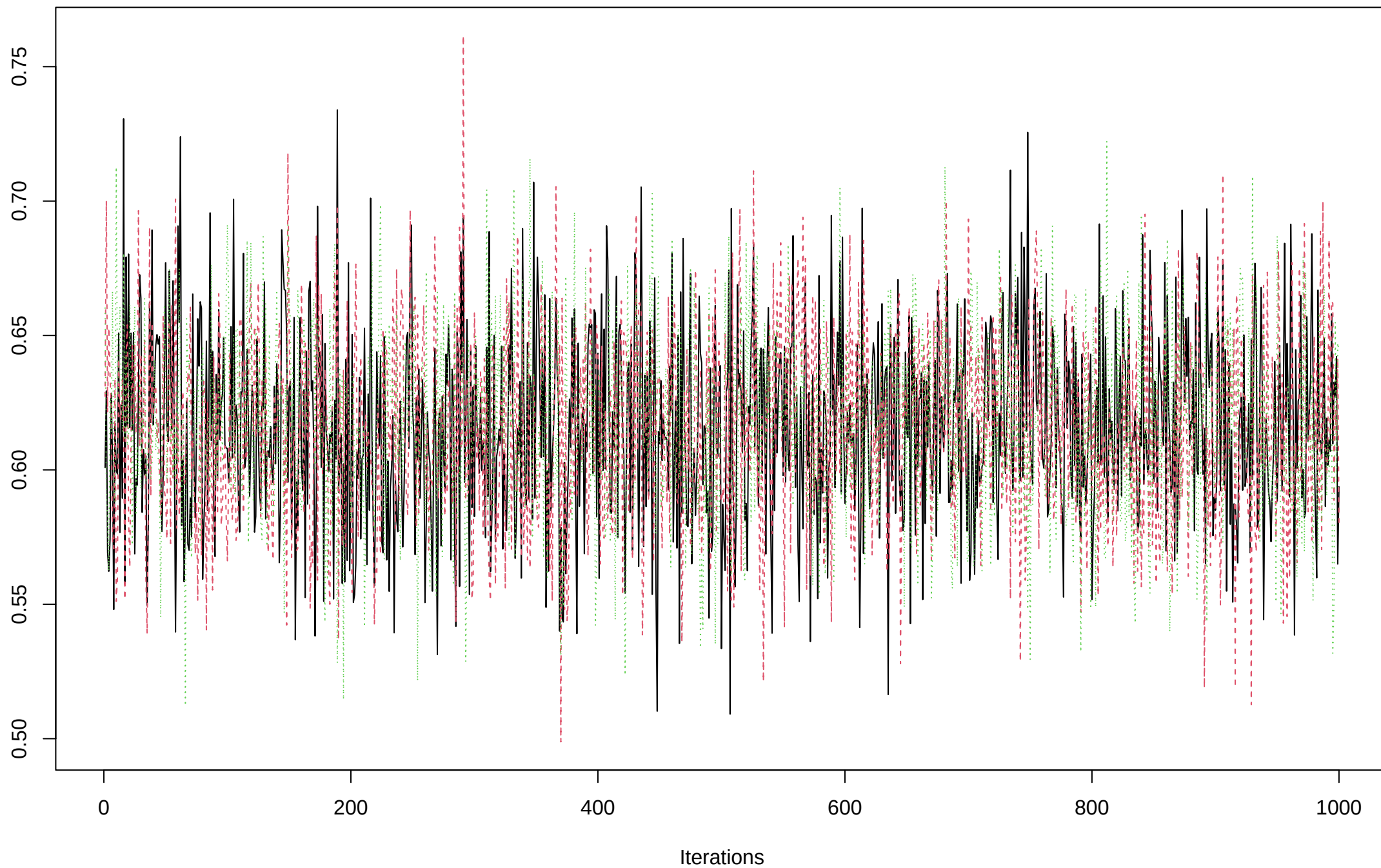
Trace of spring
