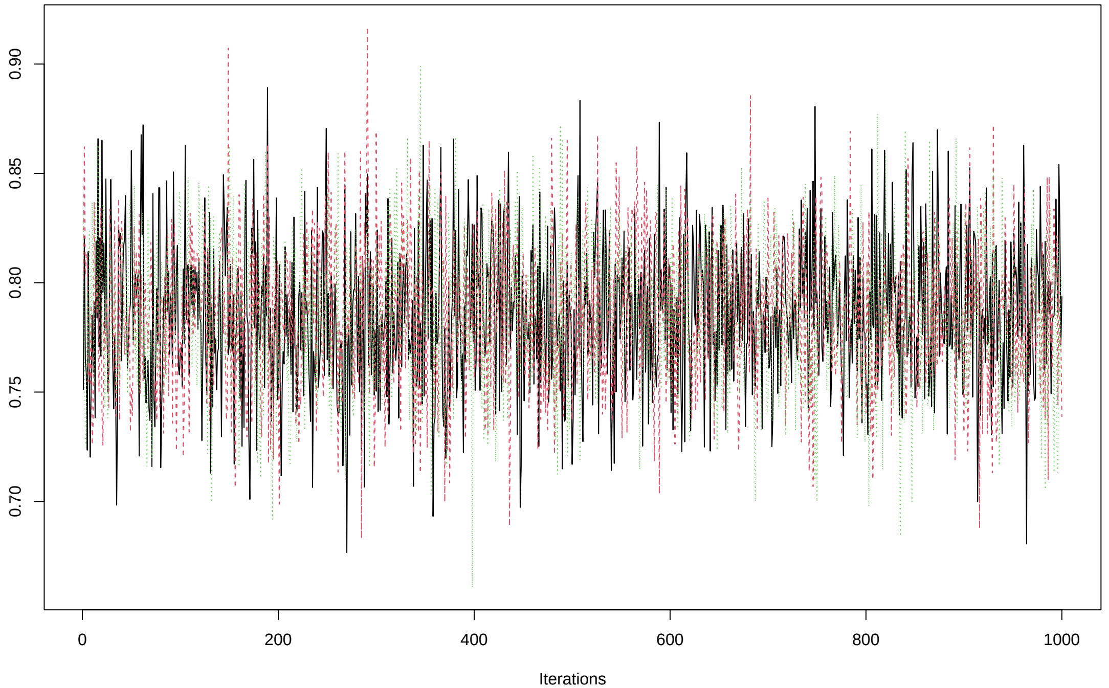
Trace of fall
