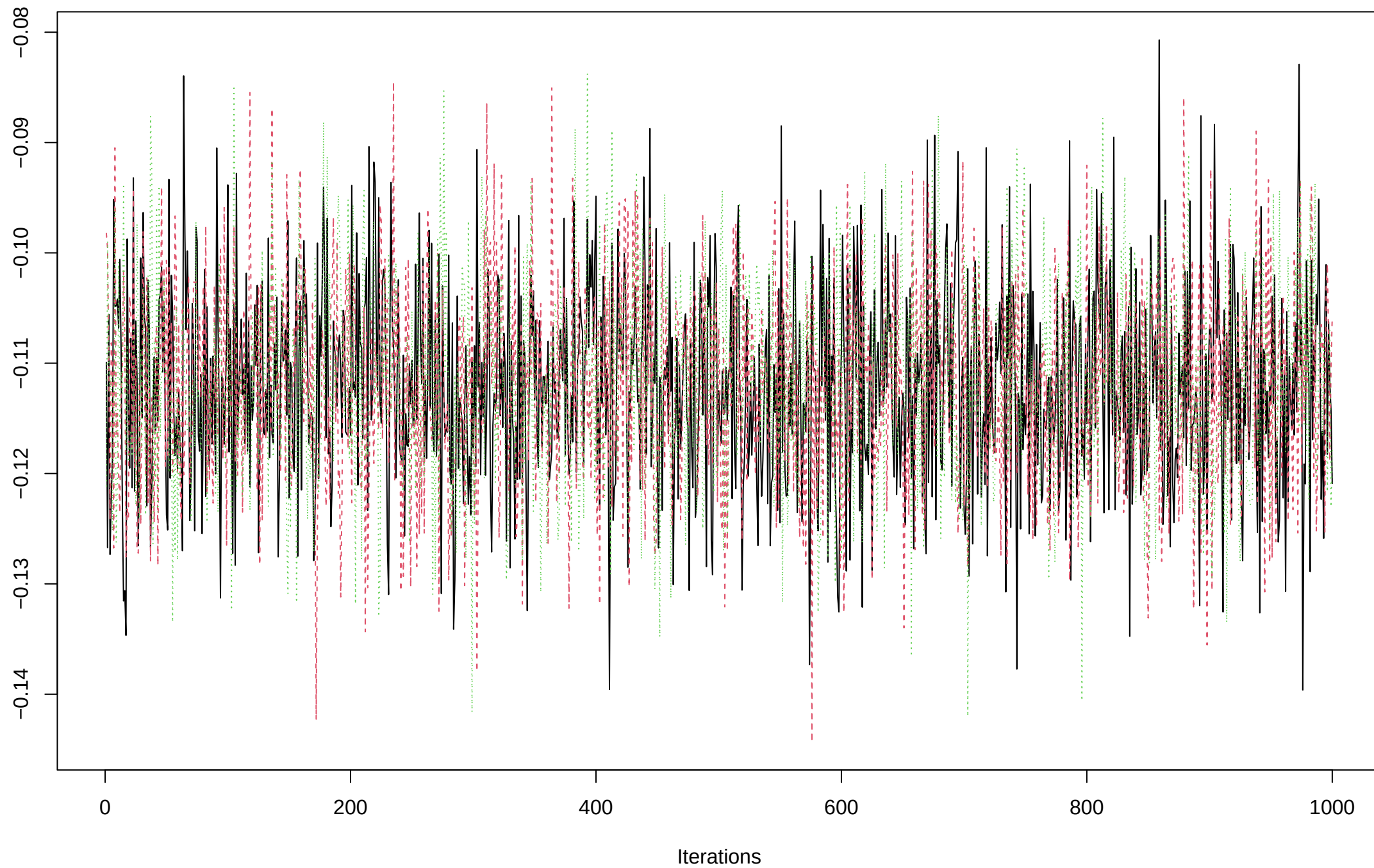
Trace of PSTot
