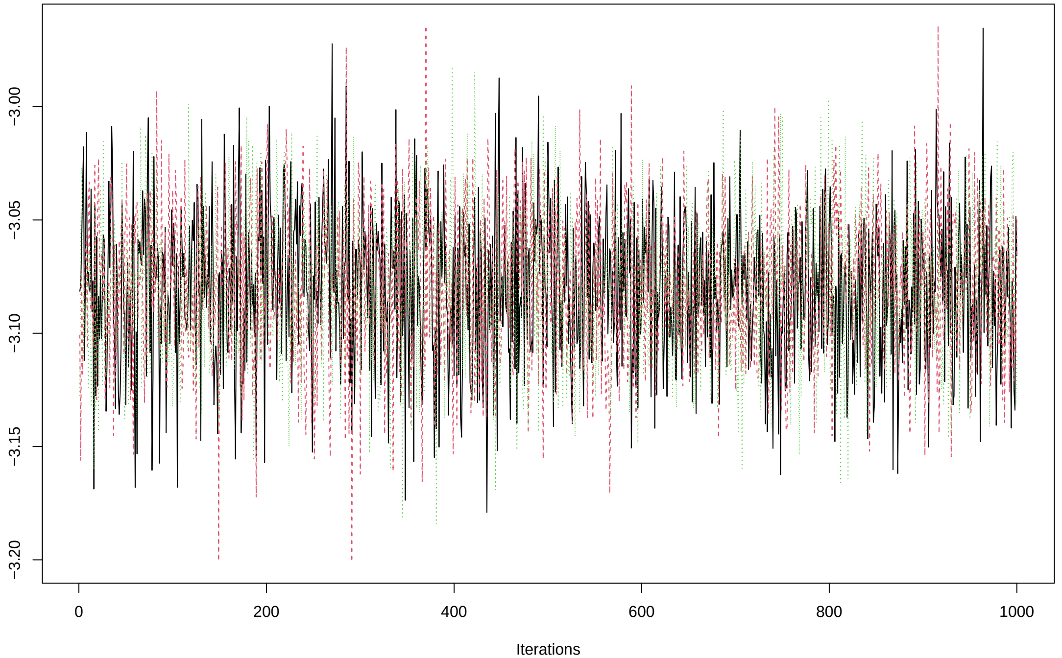
Trace of intercept
