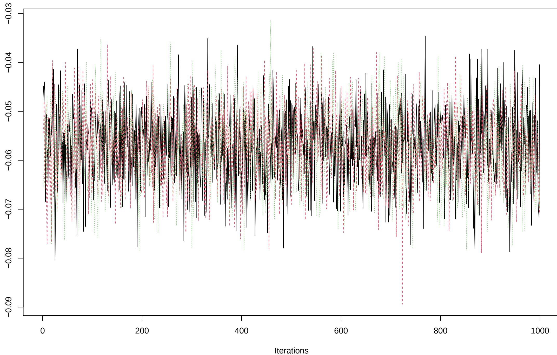
Trace of TAAve
