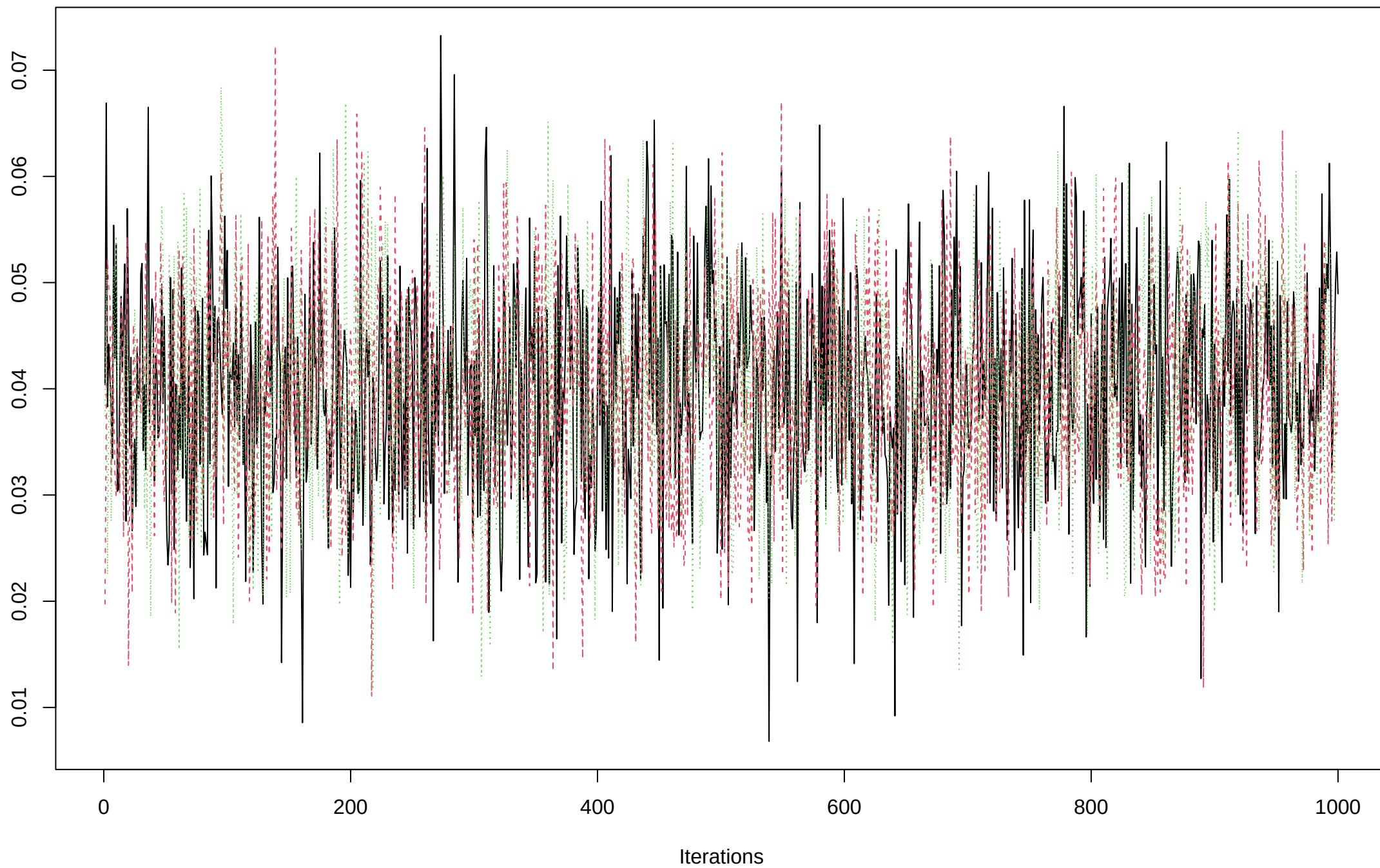
Trace of TShotweek
