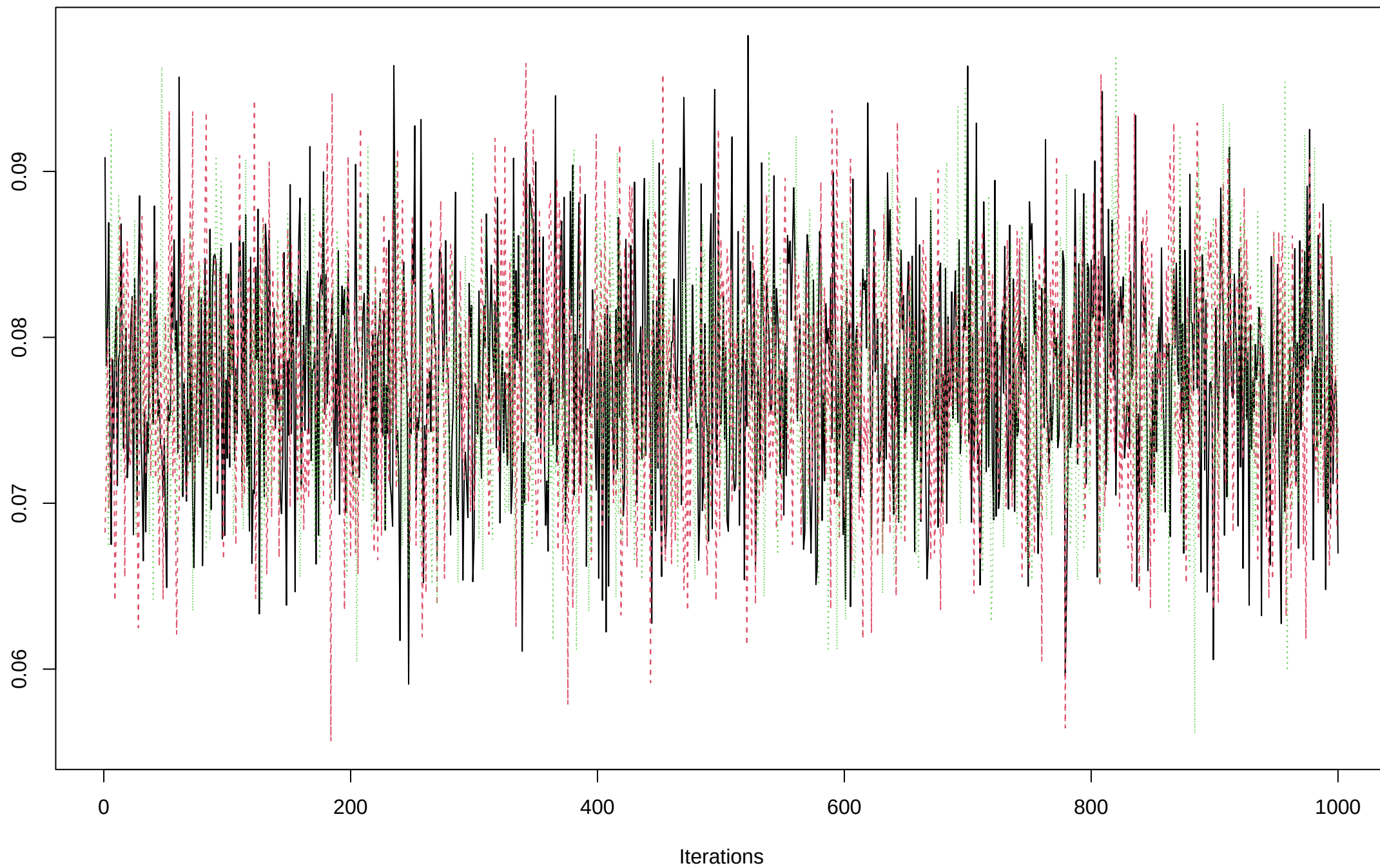
Trace of aao
