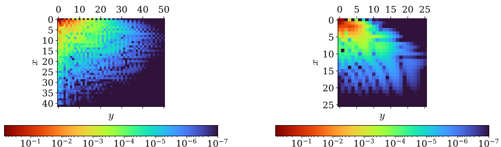
(a) |a_{xy}| on the plasma boundary of an NCSX stellarator with N_{\text{FP}} = 3 .
