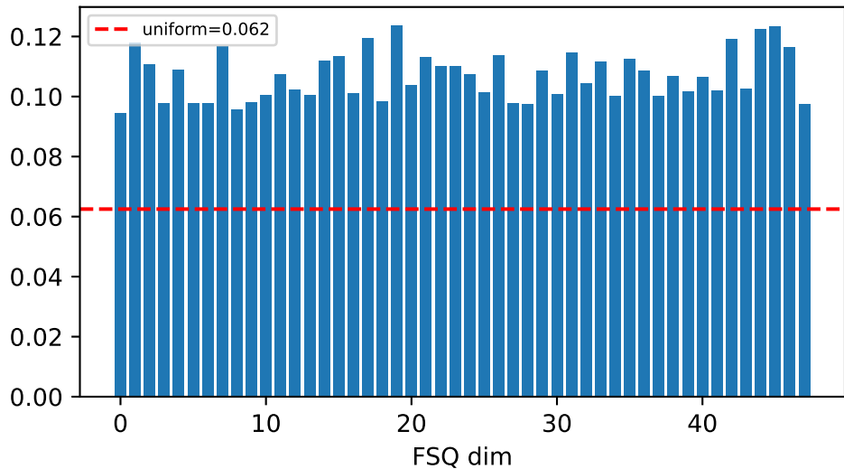
ece: per-dim top-1 level coverage
