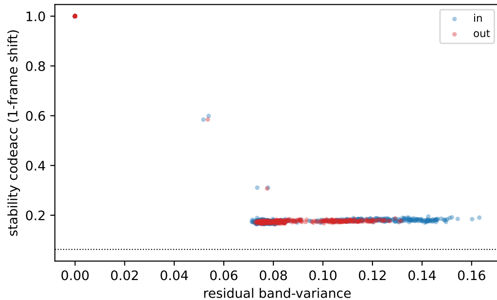
co2: stability vs activity
