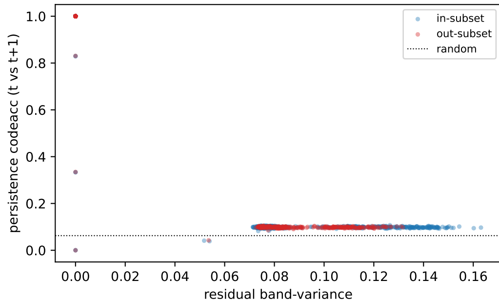
co2: what is 'easy'? codeacc vs activity
