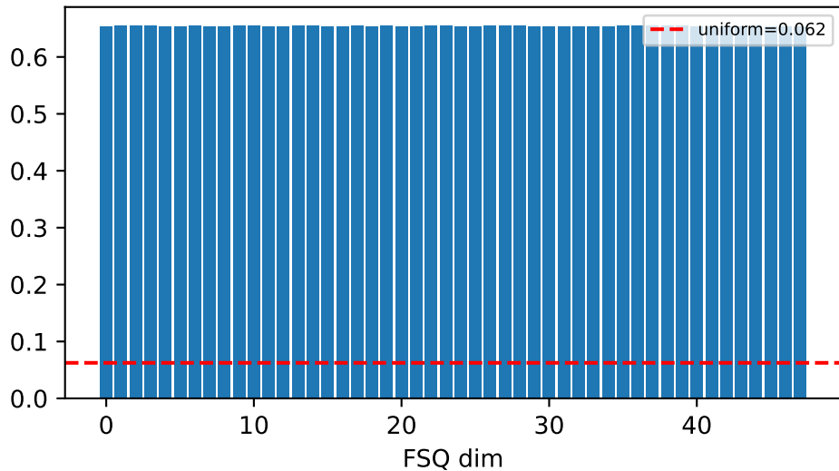
mhr: per-dim top-1 level coverage
