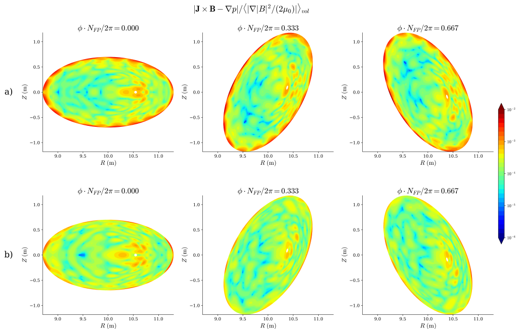
Figure 2: The ideal MHD force error normalized by volume-averaged magnetic plasma pressure for (top) the Poincaré solution and (bottom) the LCFS solution of the HELIOTRON device with N_{fp} = 19 . The errors are plotted for 3 equispaced toroidal angles between 0 and 2\pi/N_{fp} in log scale, over the range 10^{-2} to 10^{-6} .
