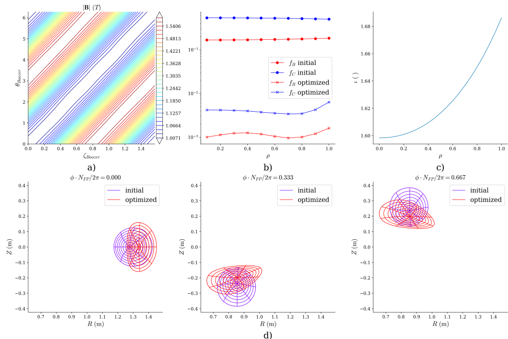
Figure 4: a) |B| level sets in Boozer coordinates for \rho = 1 surface, b) Quasisymmetry errors before and after optimization with respect to 2 different metric where f_B is the traditional definition using the Boozer transform and f_c is defined in Equation 3.6 c) Rotational Transform of the optimized equilibria, d) The flux surfaces of the initial and optimized equilibrium.
