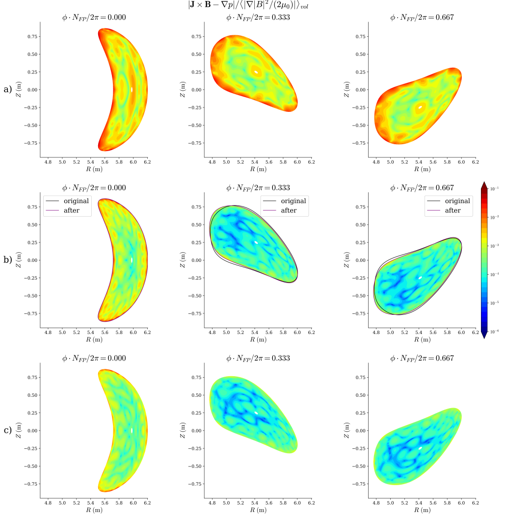
Figure 3: The ideal MHD force error normalized by volume-averaged magnetic plasma pressure (a) for LCFS solution, (b) Poincaré solution, (c) Poincaré solution fed back to LCFS solver of the W7-X device. All of them are solved for \text{ftol}=1\text{E-}3 , which is the relative decrease in the objective value between 2 consecutive iterations. The errors are plotted for 3 equispaced toroidal angles between 0 and 2\pi/N_{fp} . Part (b) additionally shows the LCFS of both equilibria for comparison.
