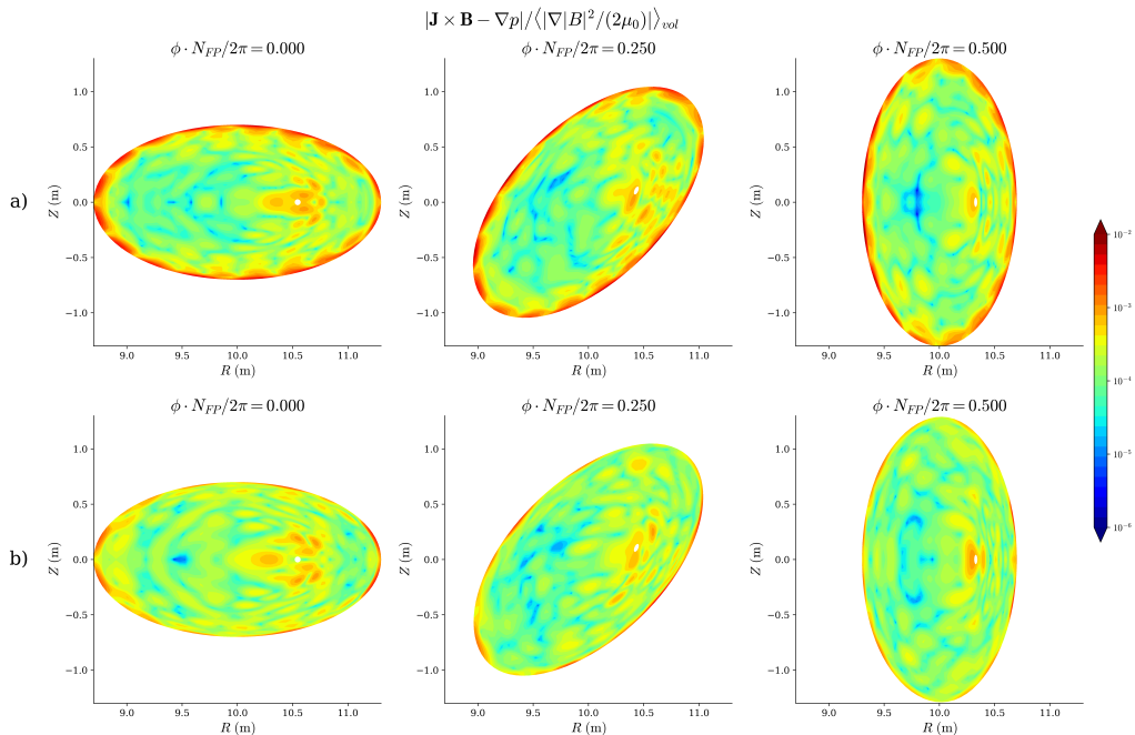
Figure 2: The ideal MHD force error normalized by volume-averaged magnetic pressure for (top) the LCFS solution and (bottom) the Poincaré solution of the HELIOTRON device with N_{fp} = 19 . The errors are plotted in log scale for 3 equispaced toroidal angles between 0 and \pi/N_{fp} , over the range 10^{-2} to 10^{-6} .
