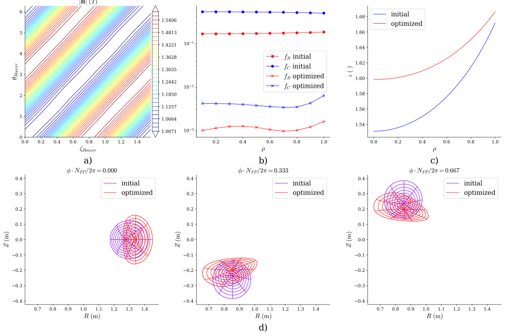
Figure 4: a) |B| level sets in Boozer coordinates for \rho = 1 surface, b) Quasisymmetry errors before and after optimization with respect to 2 different metrics where f_B is the traditional definition using the Boozer transform and f_C is defined in Equation 3.6 c) Rotational Transform of the initial and optimized equilibria, d) The flux surfaces of the initial and optimized equilibrium.
