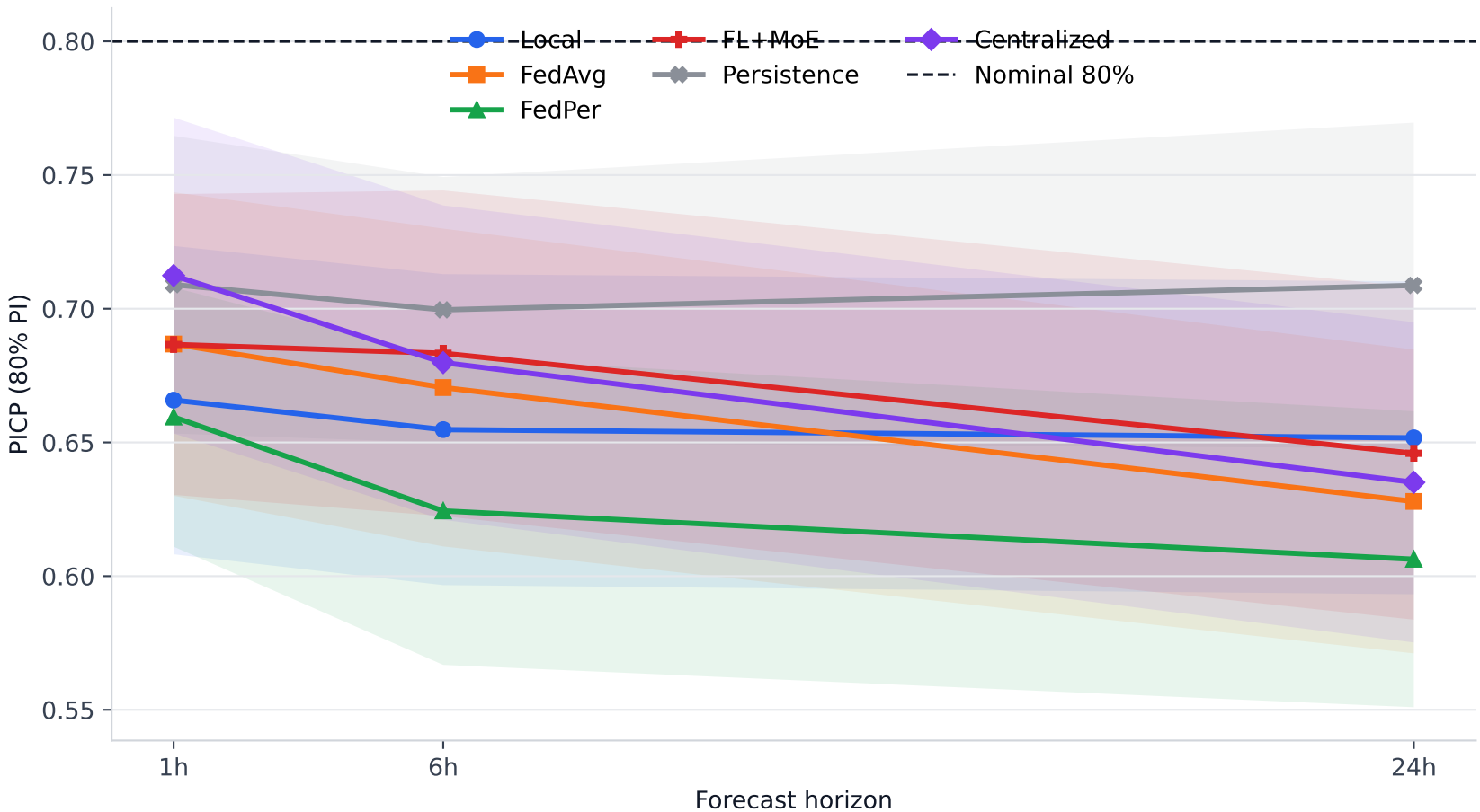
PICP (80% PI) across forecast horizons
