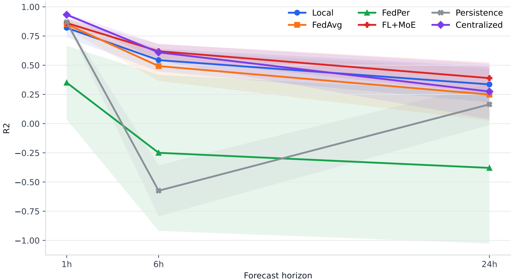
R2 across forecast horizons
