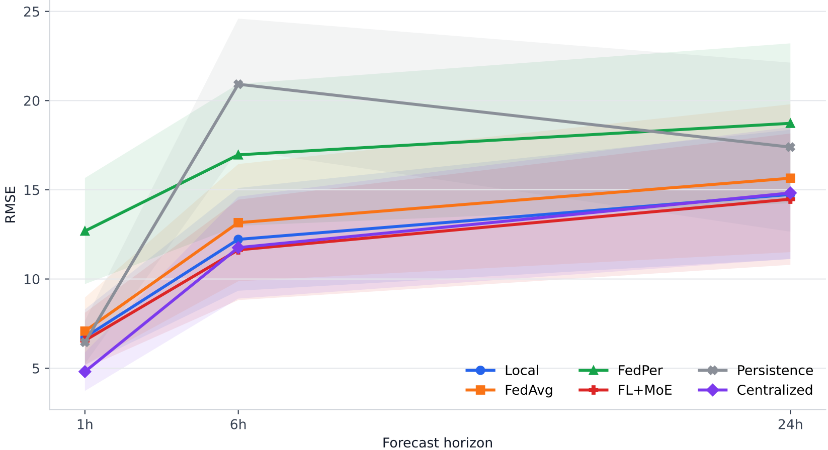
RMSE across forecast horizons
