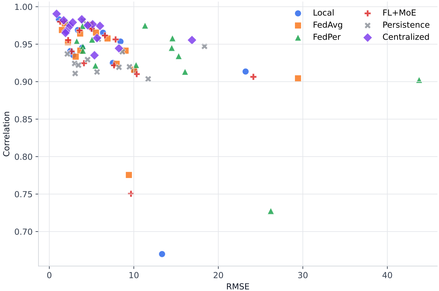
RMSE-Correlation tradeoff (1h)
