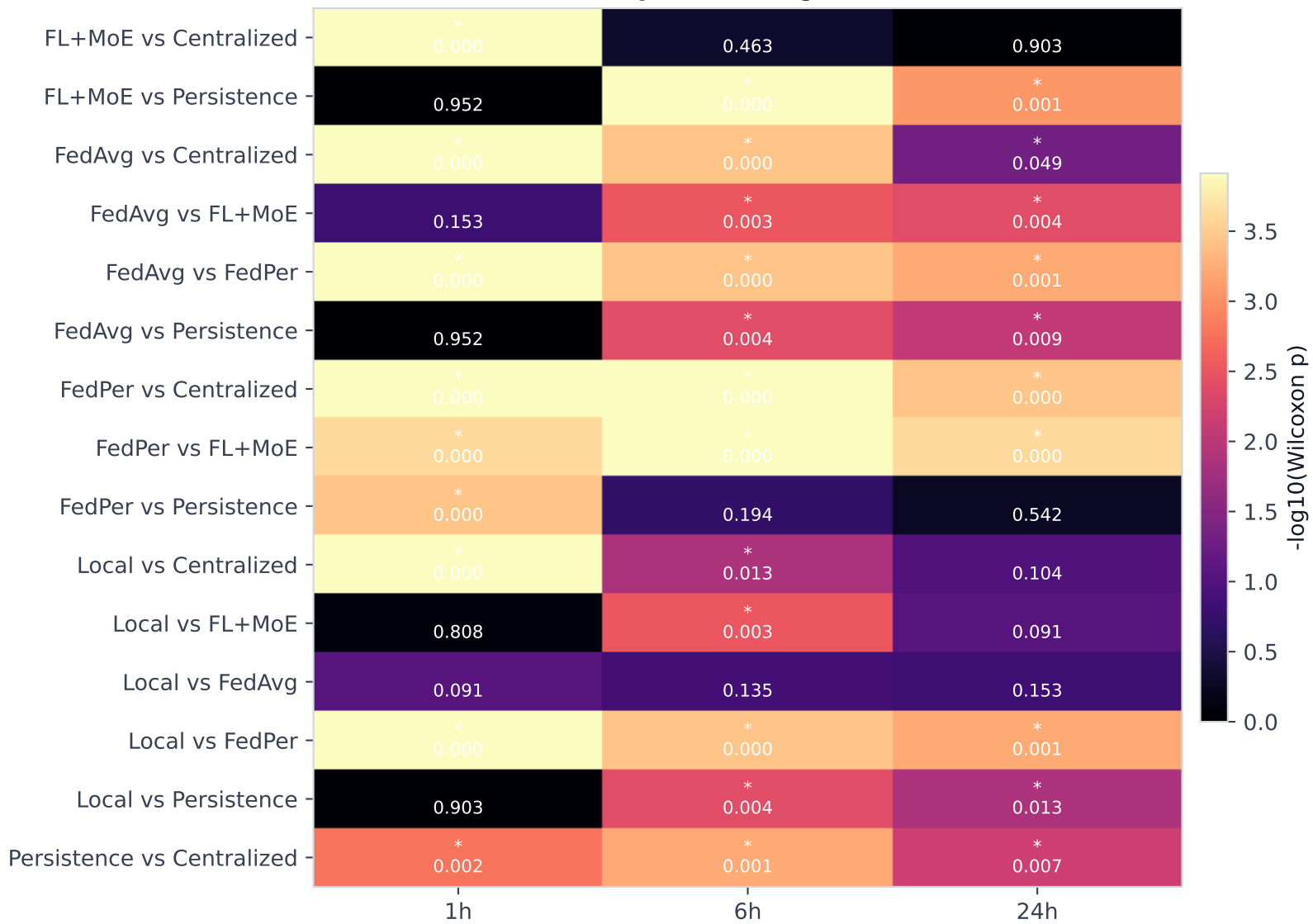
RMSE pairwise significance
