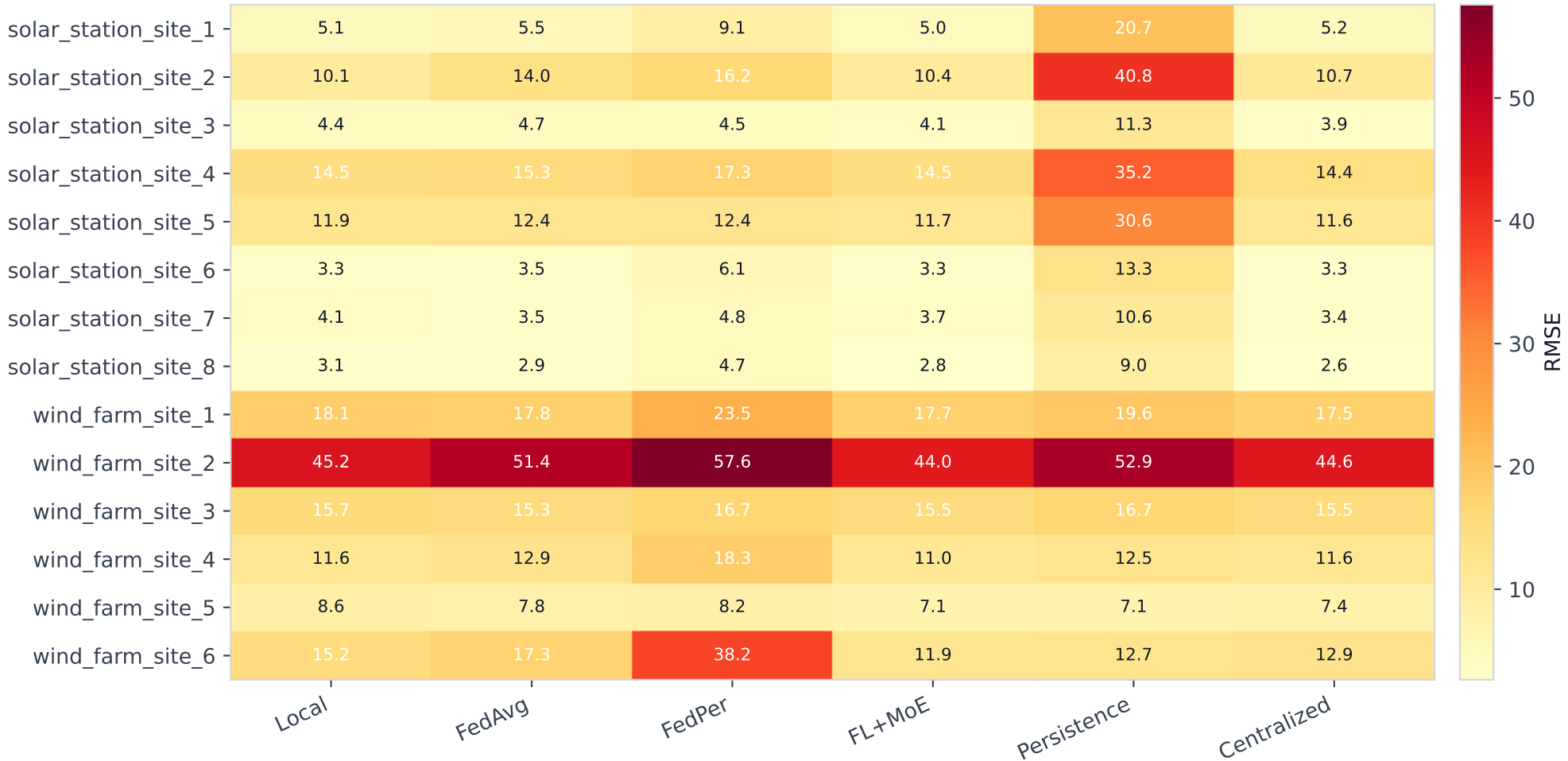
Per-site RMSE heatmap (6h)
