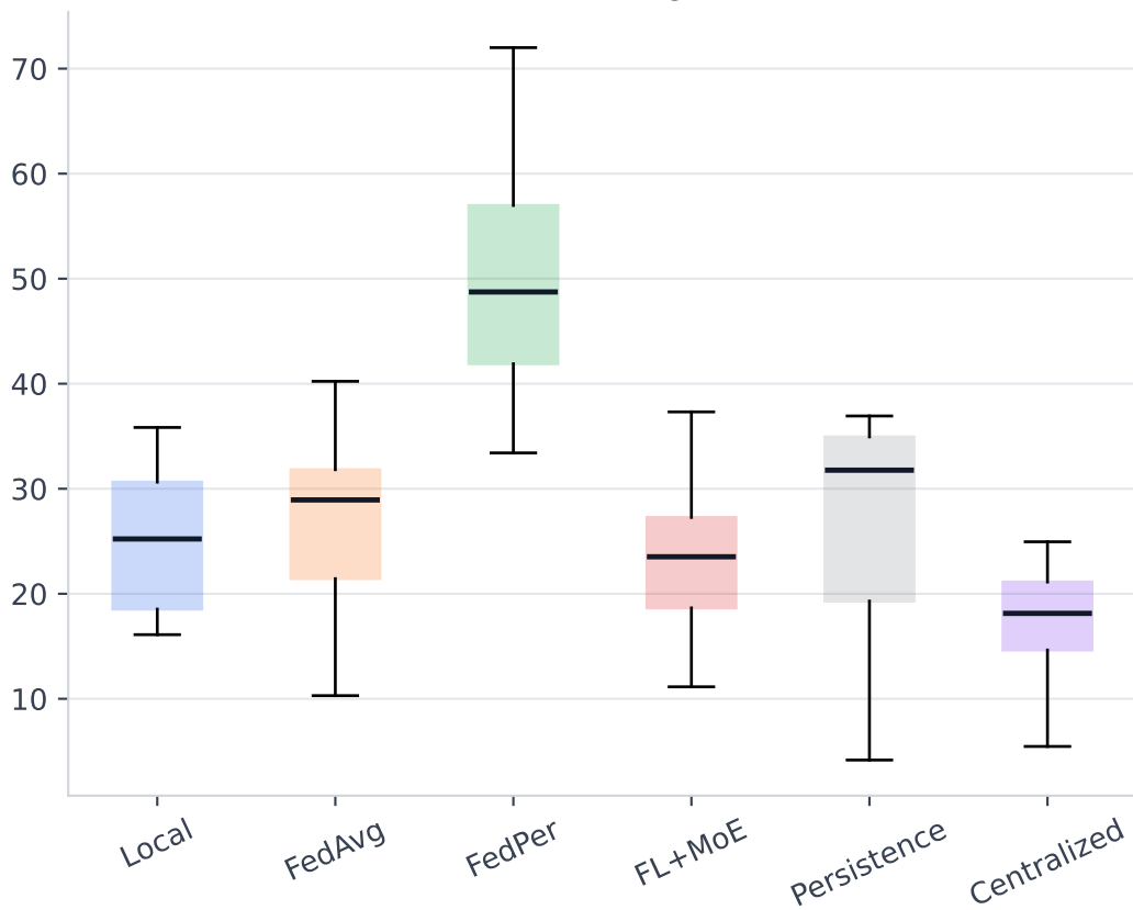
WAPE (%) @ 1h
