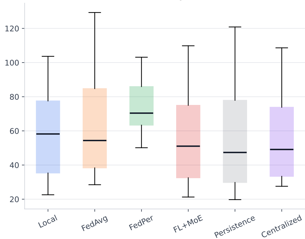
WAPE (%) @ 24h
