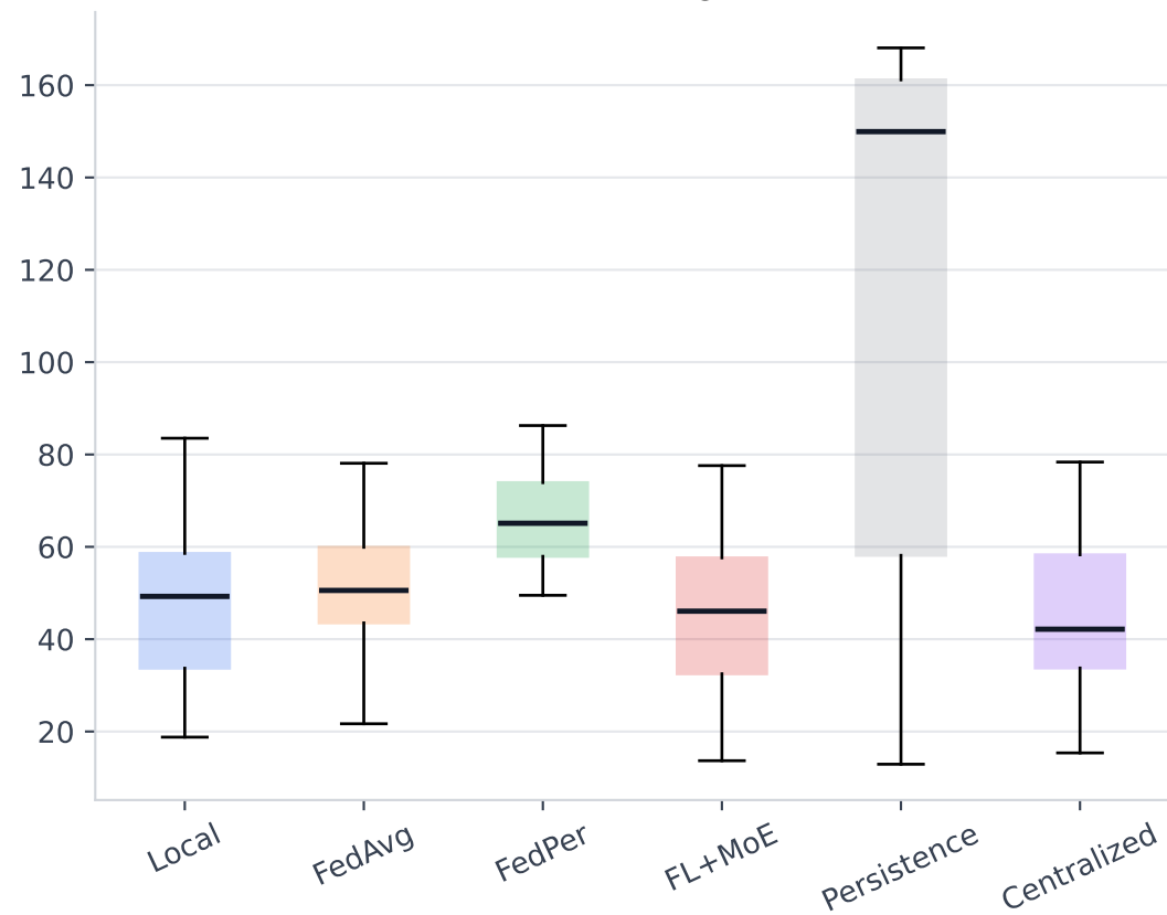
WAPE (%) @ 6h
