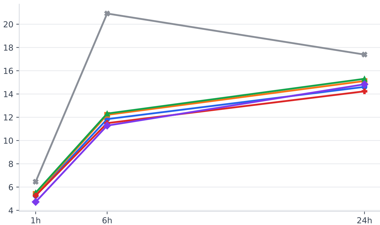
PICP (80% PI)
