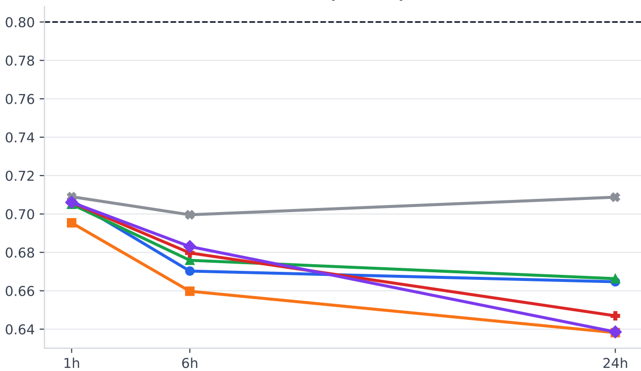
PICP (80% PI)
