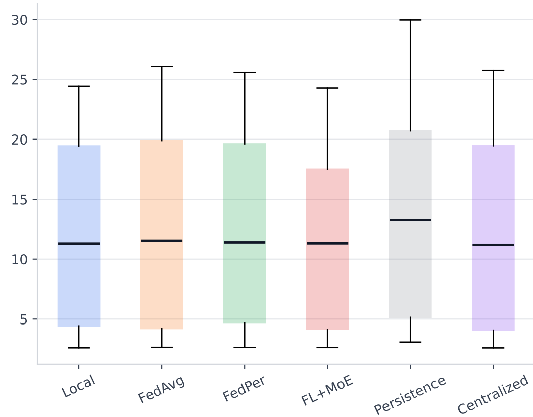
RMSE @ 24h
