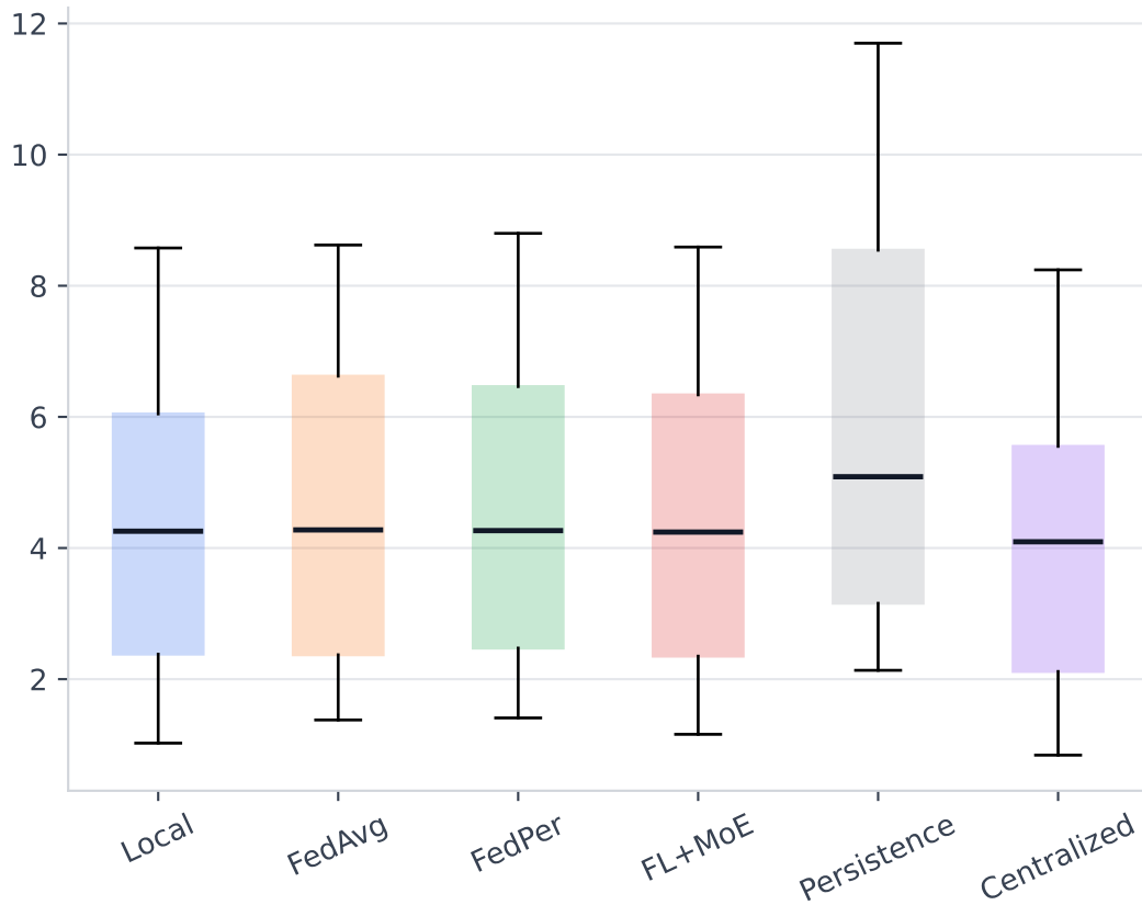
RMSE @ 1h
