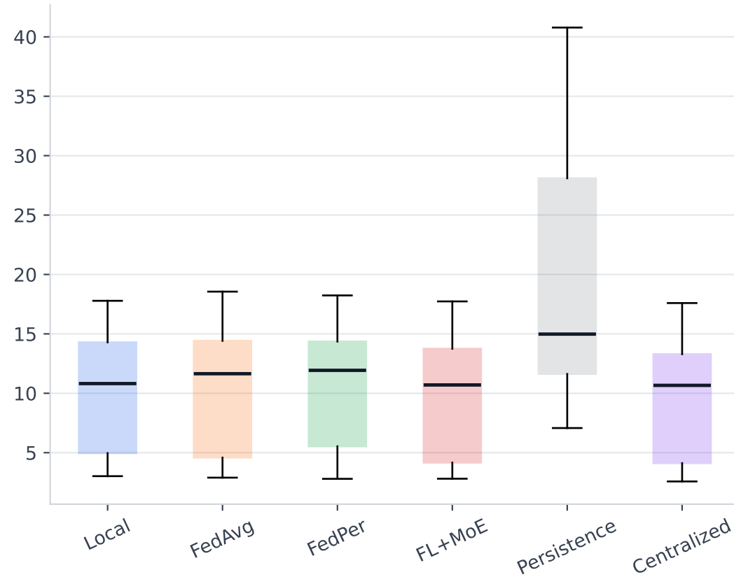
RMSE @ 6h
