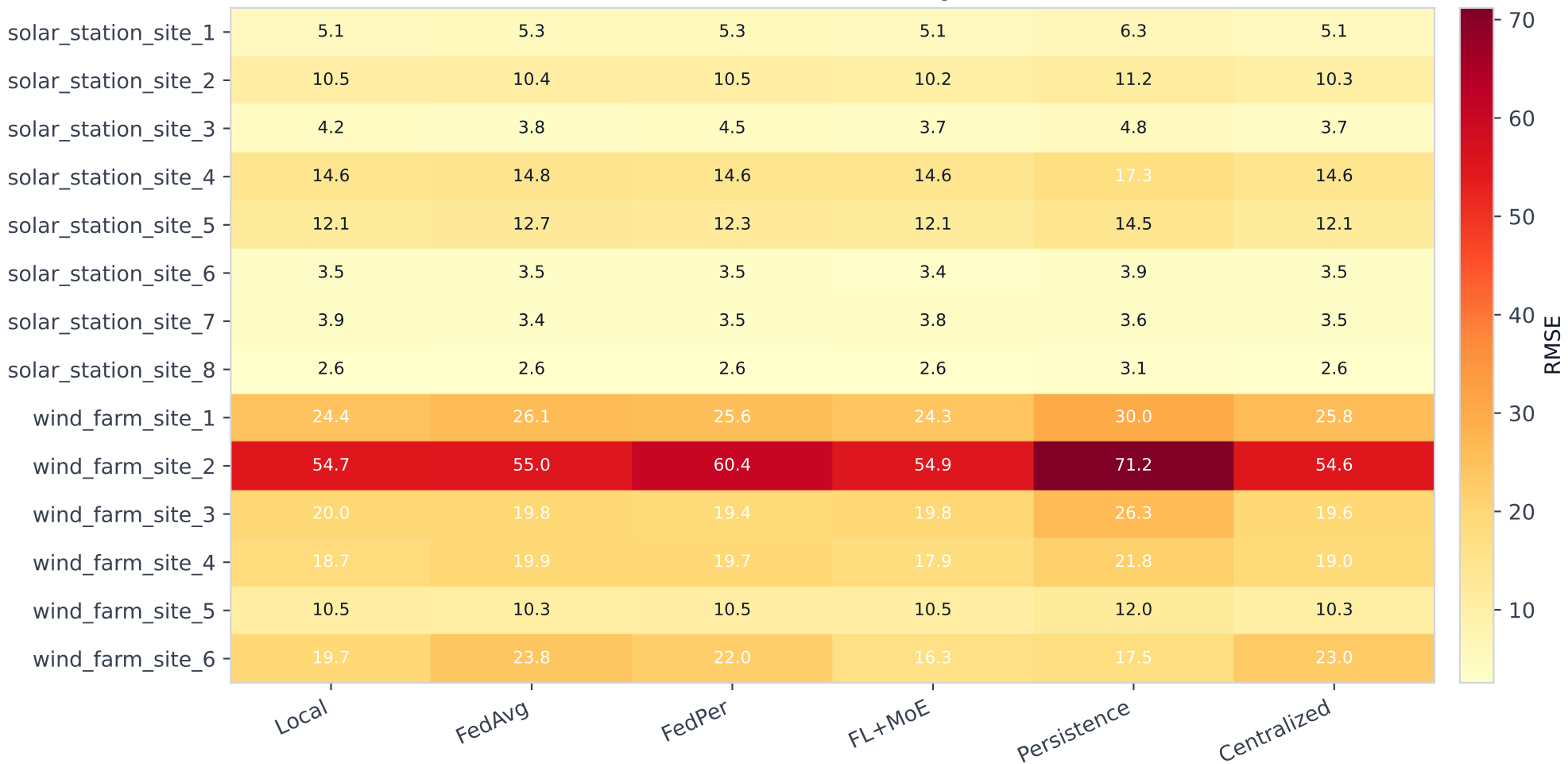
Per-site RMSE heatmap (24h)
