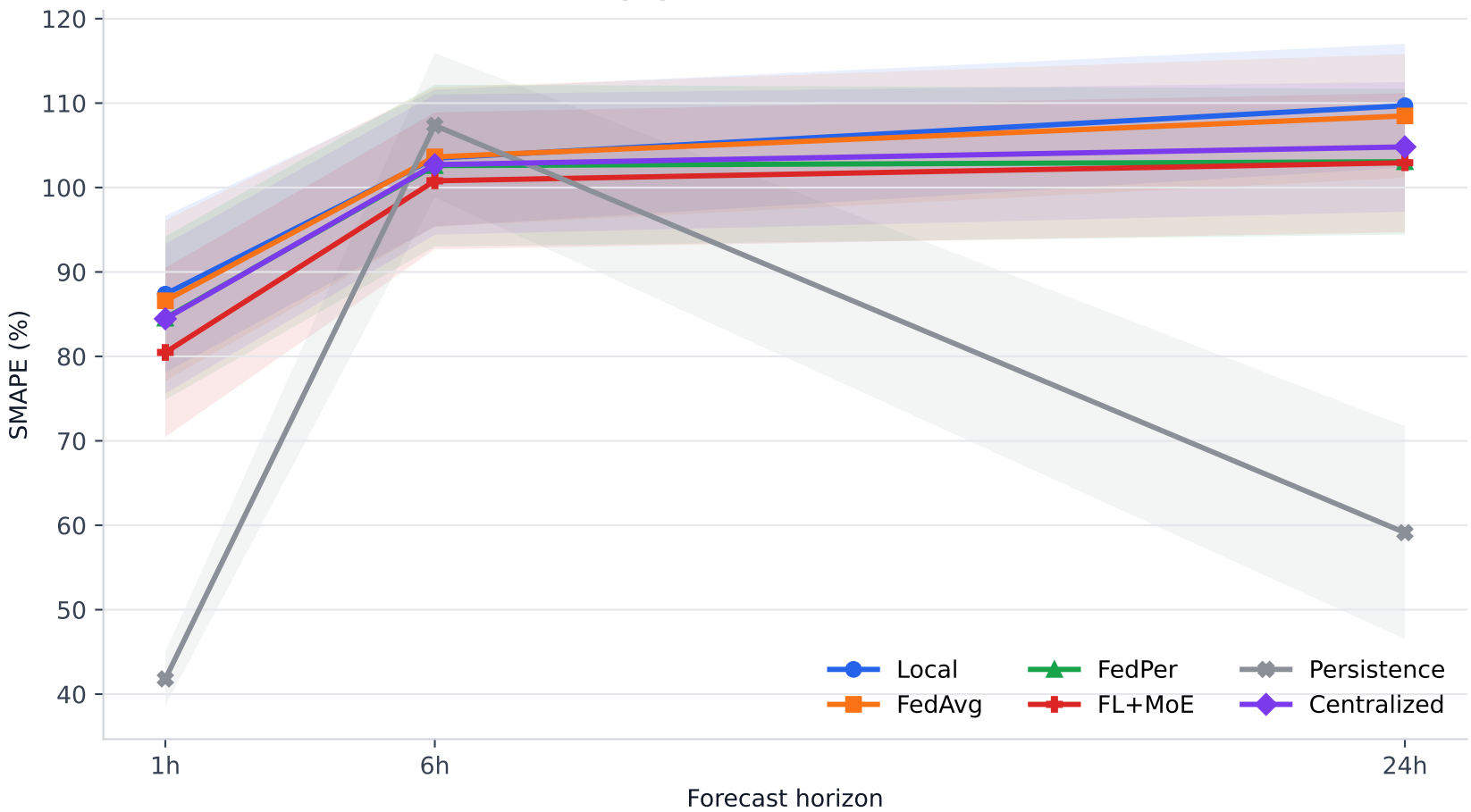
SMAPE (%) across forecast horizons
