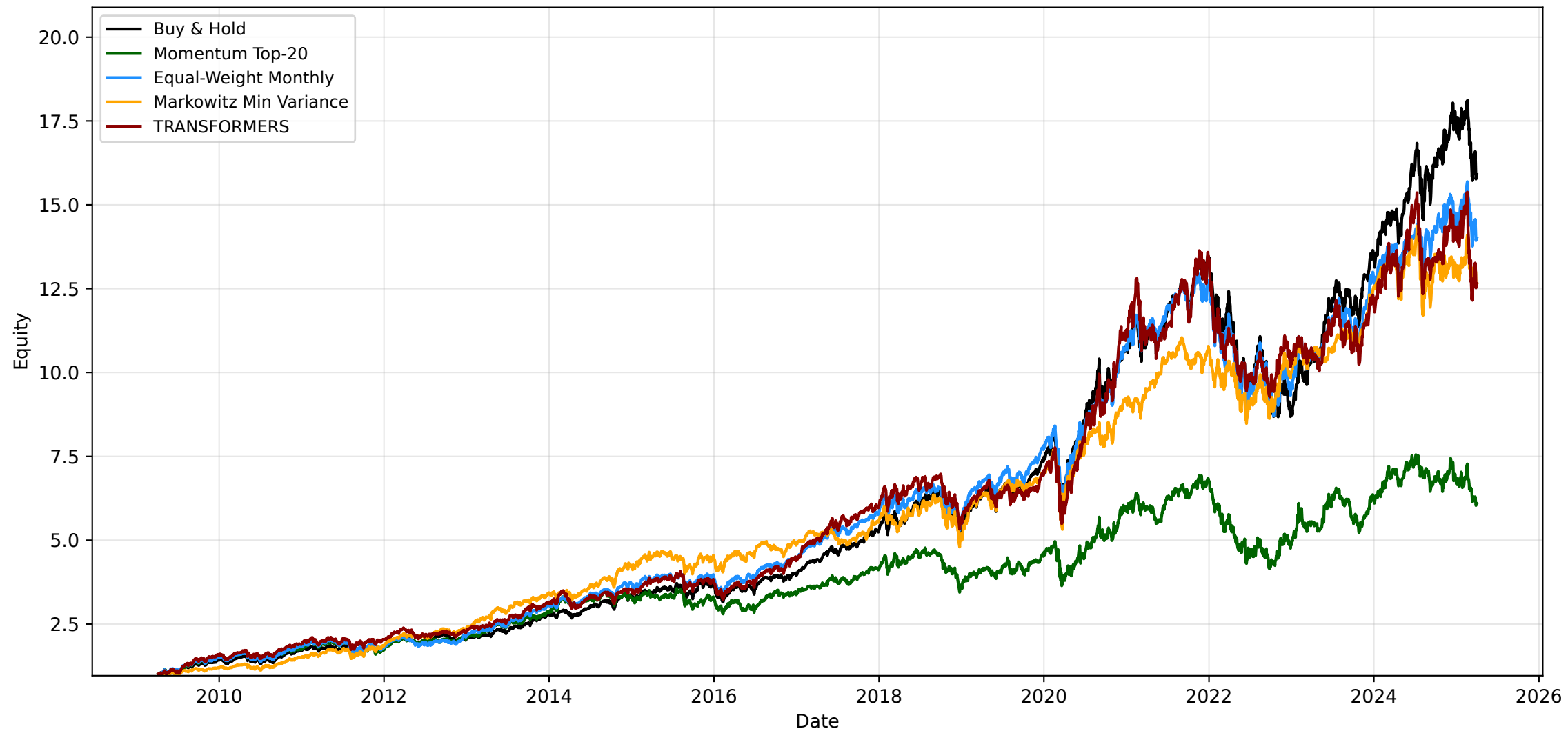
Panel C: RL with Transformers
