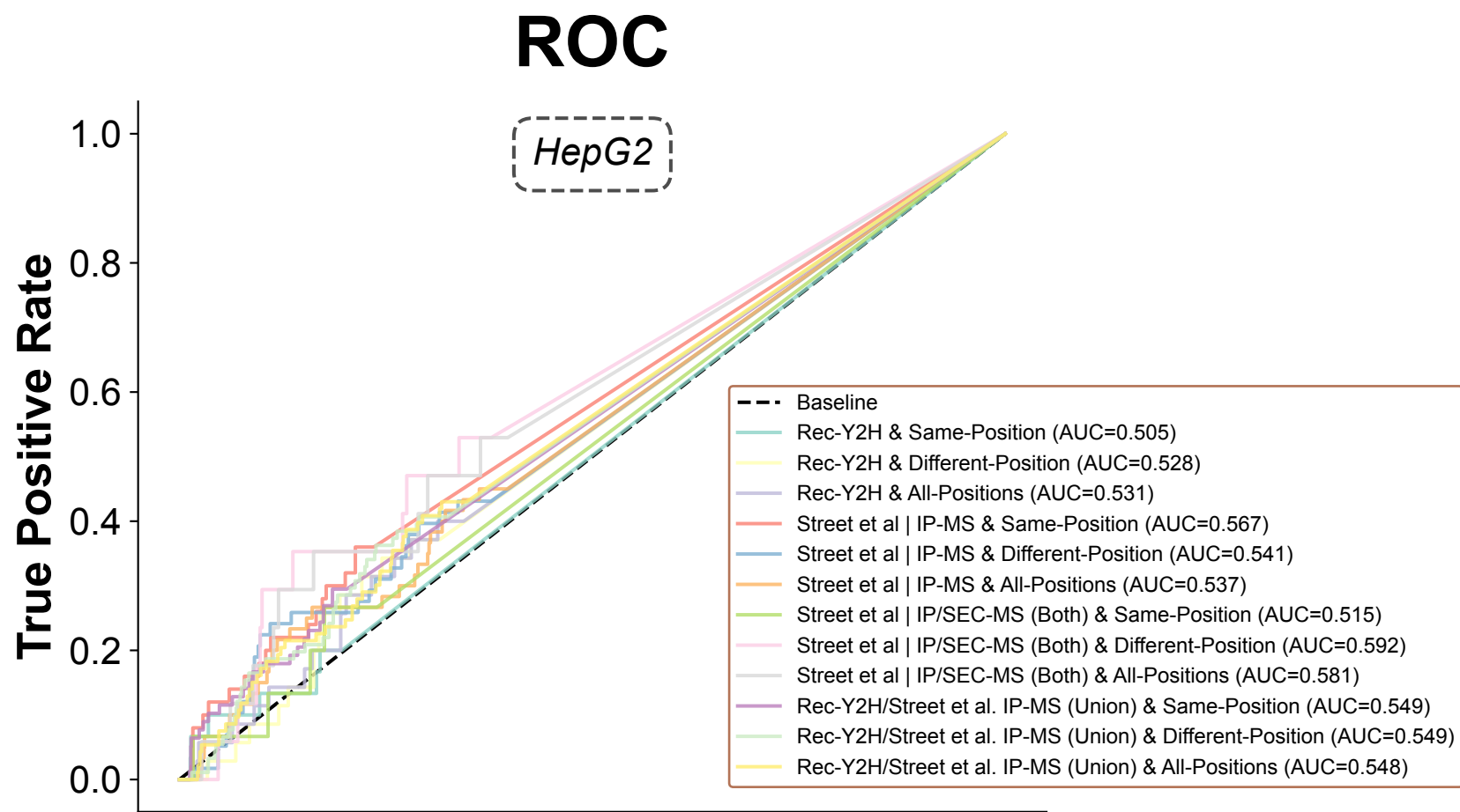
RBP-SPECIFIC_MAX_VALUE: ROC and PRC Curves by Cell Line and PPI Source & PPI Type
