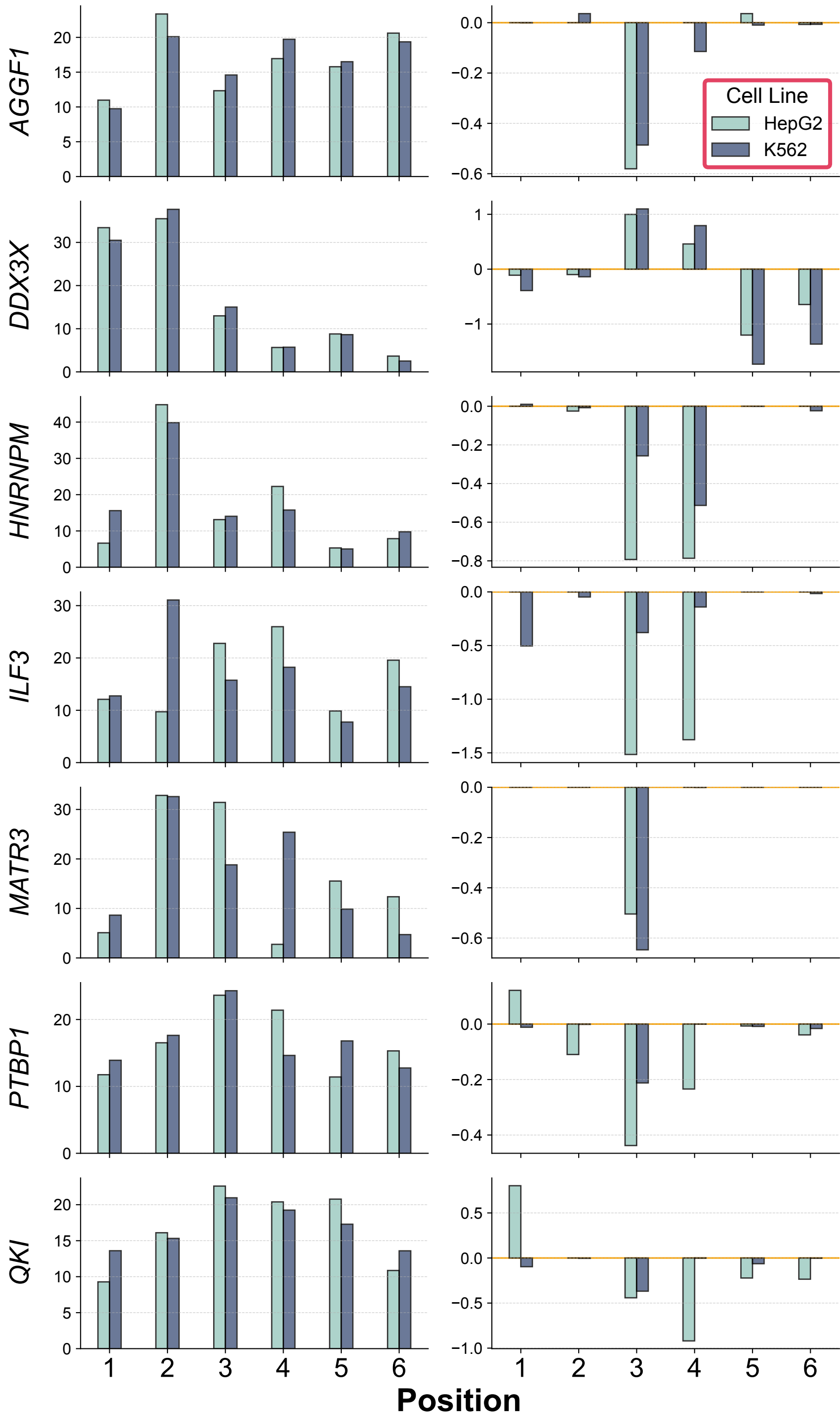
RBP Positional Preference (% RBP Binding at Position)
