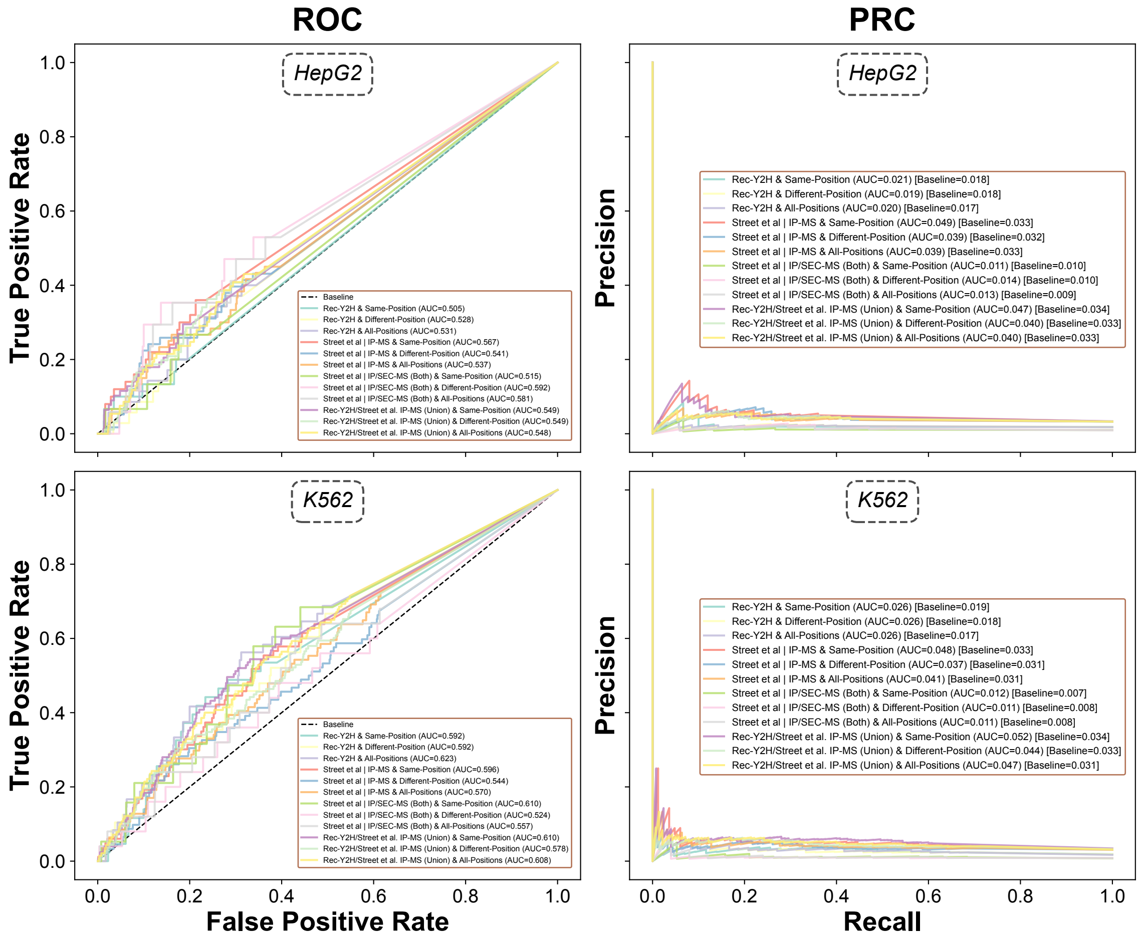
RBP-SPECIFIC_MAX_VALUE: ROC and PRC Curves by Cell Line and PPI Source & PPI Type
