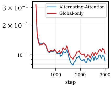
camera loss
