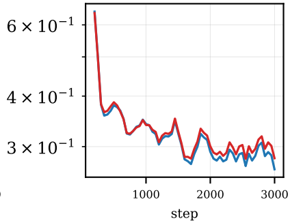
point regression
