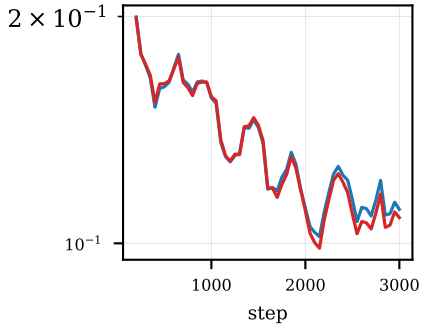
depth regression
