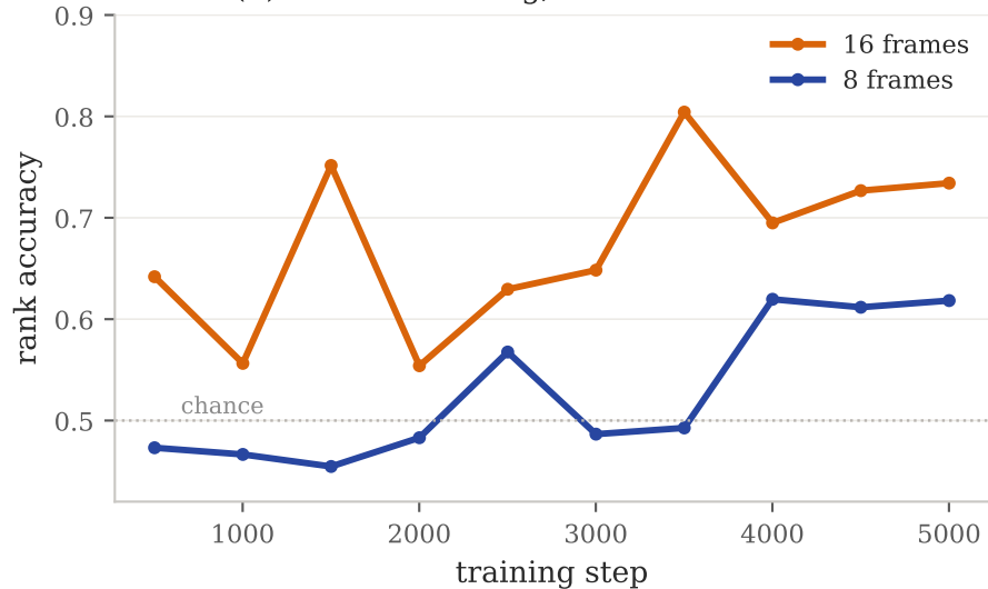
(b) DROID ranking, with demonstration
