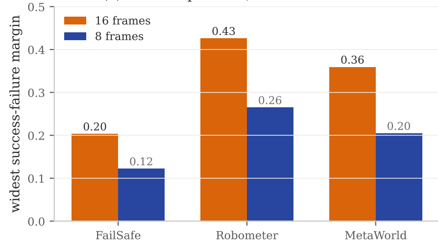
(a) score separation, with demonstration
