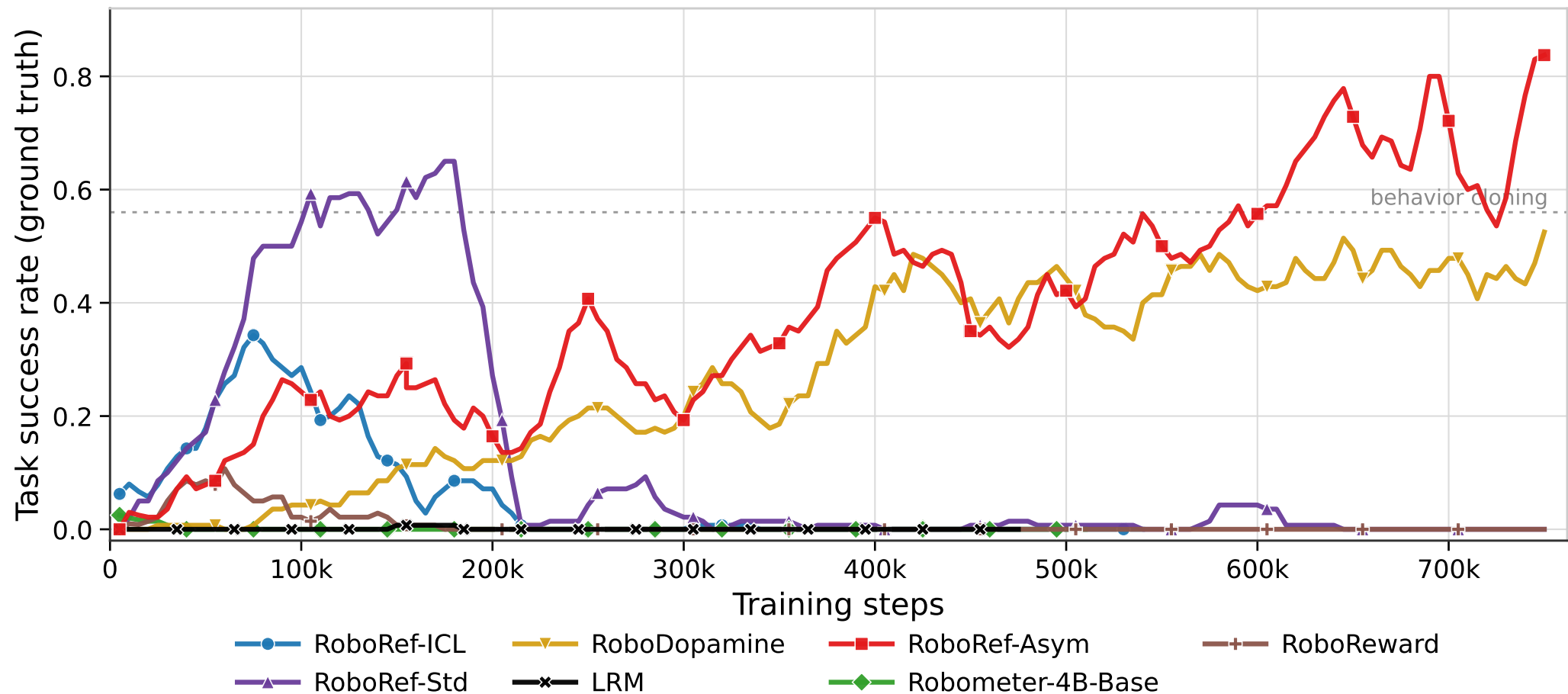
Robomimic IBRL (PickPlace-Can): policy success by VLM reward model (single seed)
