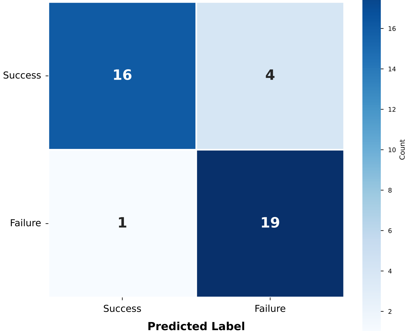
Confusion Matrix: RoboReward-8B at 10 FPS (Best Performance - Mixed Dataset)
