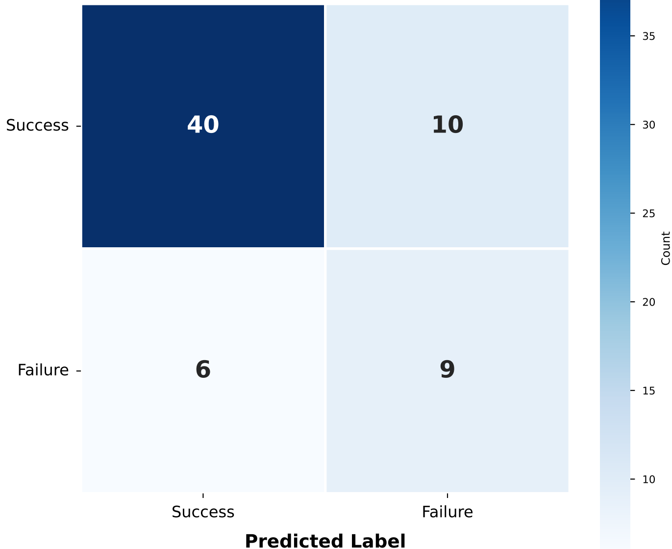
Confusion Matrix: RoboReward-8B at 60 FPS (Best Performance)
