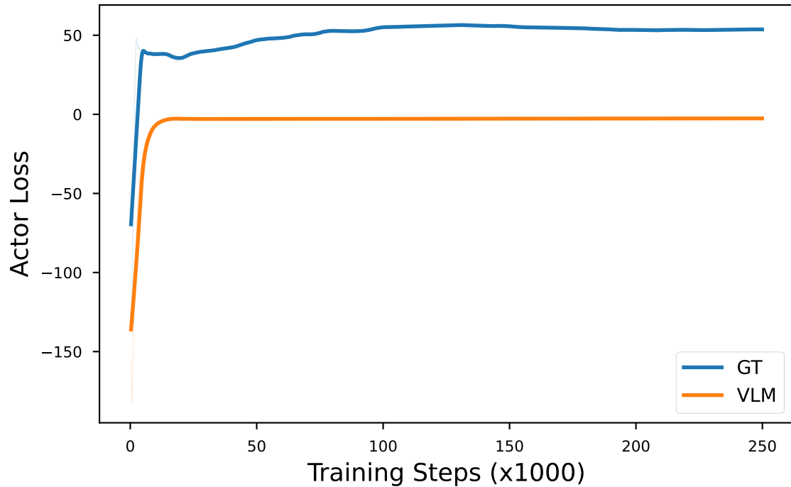
Actor Loss
