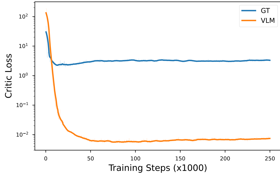
Critic Loss
