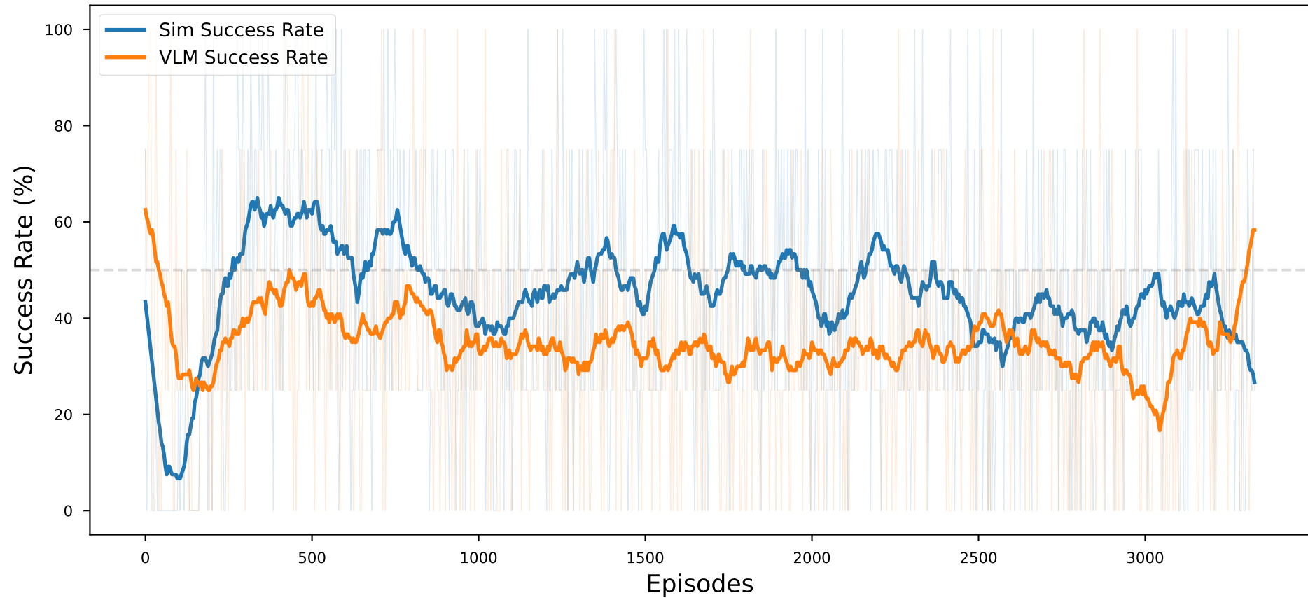
Success Rate During Training (cf. RoboReward Fig. 2)
