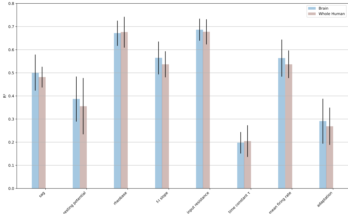
Comparison of MLPs given exclusively scGPT embedding input: one using embeddings given by the whole human model and one using embeddings given by the brain model Error bars are standard deviations across the four folds of cross-validation.
