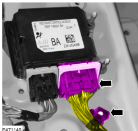
Figure 13 - PHEV
