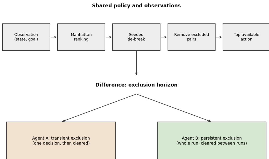
Figure 1. Shared policy and the single difference between the two agents. Both agents share the observation, Manhattan-distance ranking, seeded tie-breaking, removal of excluded state-action pairs, and selection of the top available action. They differ only in the exclusion horizon: Agent A clears an exclusion after one decision, and Agent B keeps it for the whole run.
