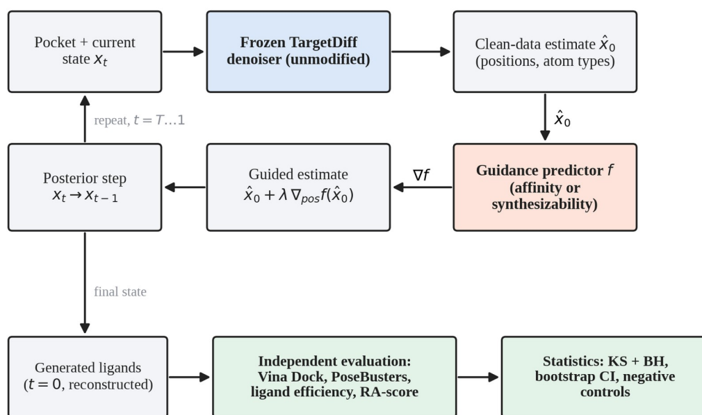
Figure 3.1 Overall pipeline. A frozen TargetDiff denoiser proposes a clean-data estimate at each reverse step; a guidance predictor's gradient with respect to atom positions modifies that estimate; and the finished molecules are evaluated by tools that are independent of the guidance predictor and analysed with corrected statistics.
