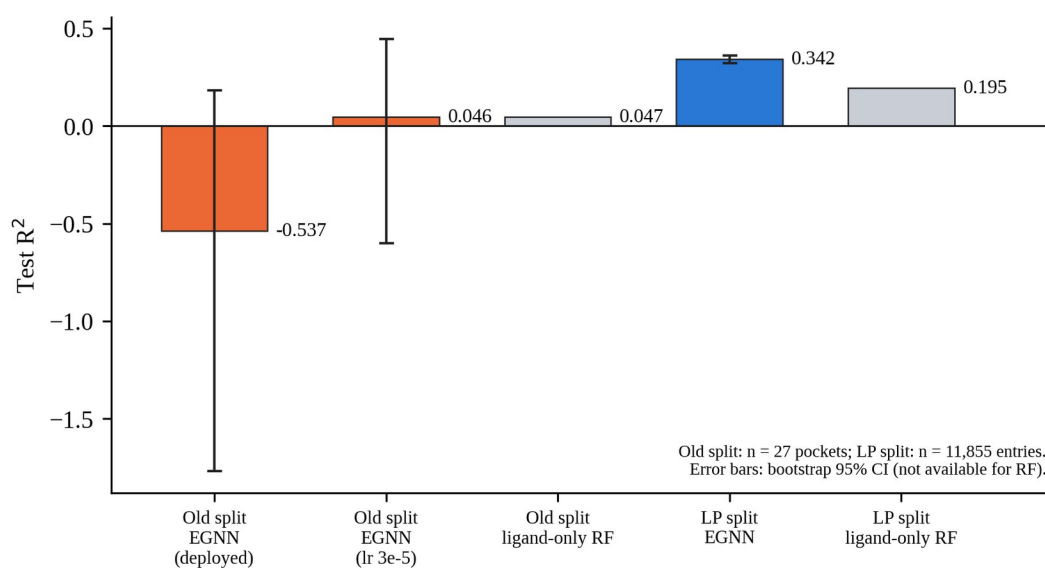
Figure 4.1 Test R^2 of the affinity predictor on the old split ( n = 27 pockets) and on the leakage-safe split ( n = 11,855 entries). Ligand-only random forests are shown in grey. Error bars are bootstrap 95% confidence intervals where available.
