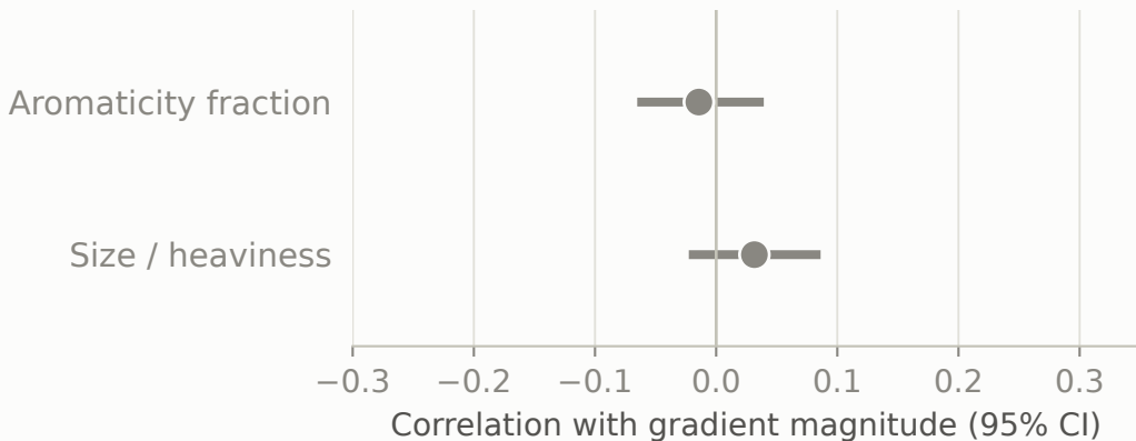
D.5 (synth guidance): neither proxy explains the failure
