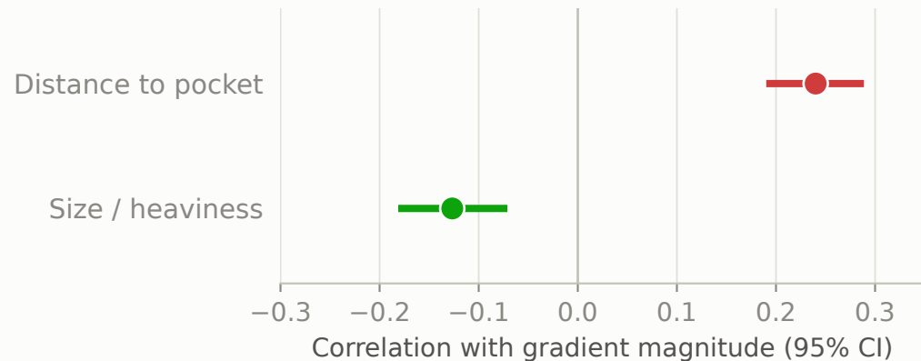
DIAG1 (affinity guidance): distance-to-pocket explains the failure
