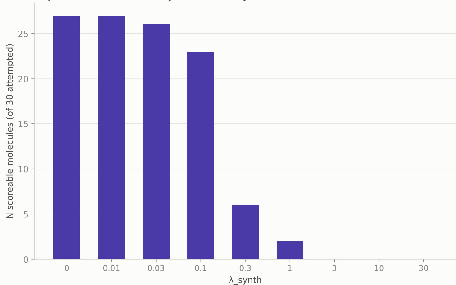
Track D: sample size collapses at higher \lambda — large point estimates beyond \lambda=0.3 rest on very few surviving molecules
