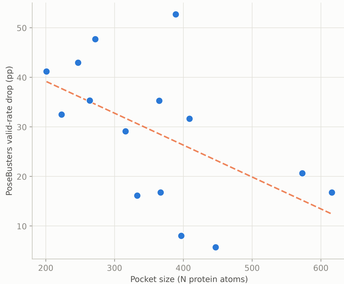
A. Smaller pockets are more susceptible Spearman r=-0.59 , 95% CI excludes 0
