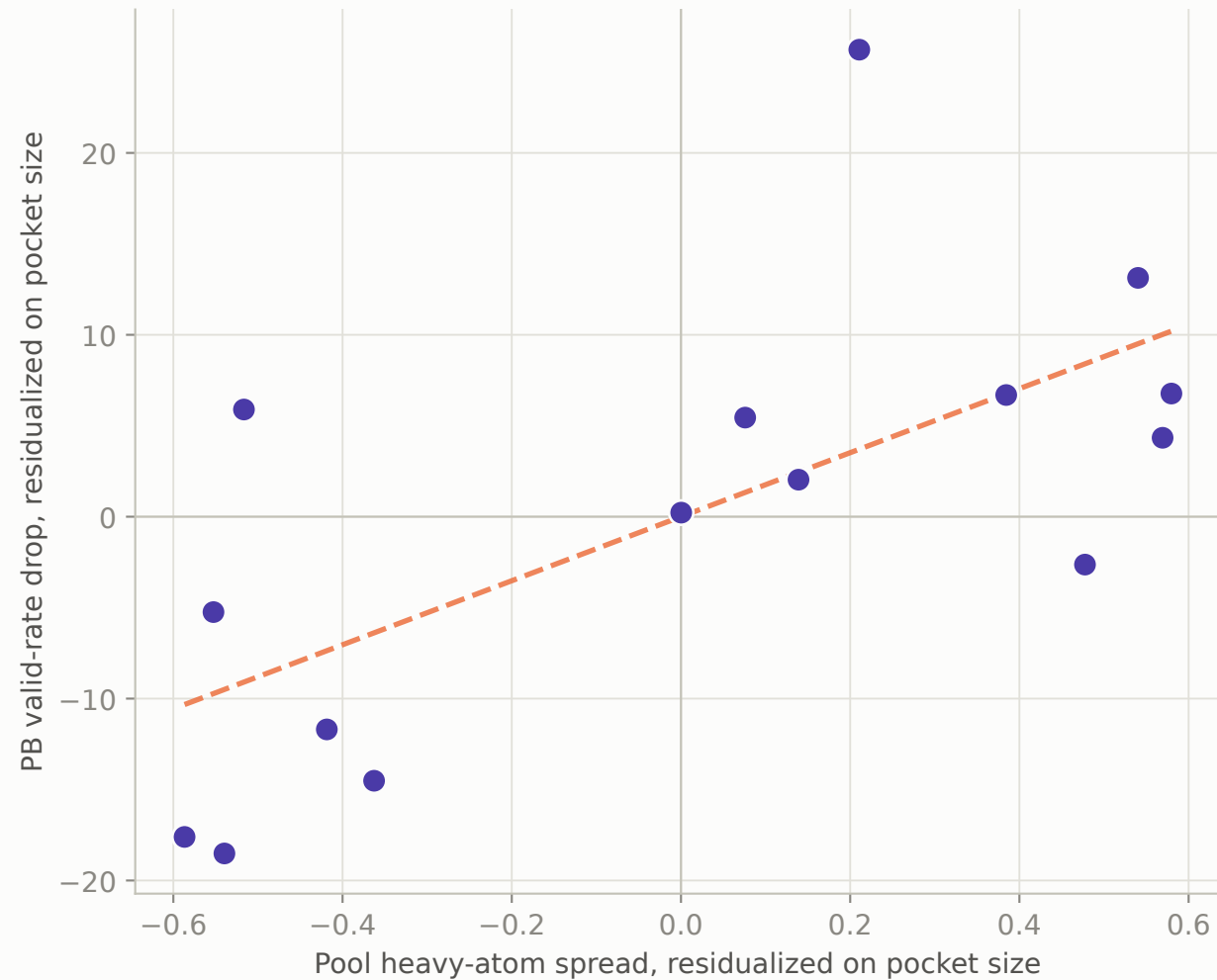
B. Wider baseline pool spread also predicts damage partial r=0.70 , 95% CI excludes 0 (independent of A)
