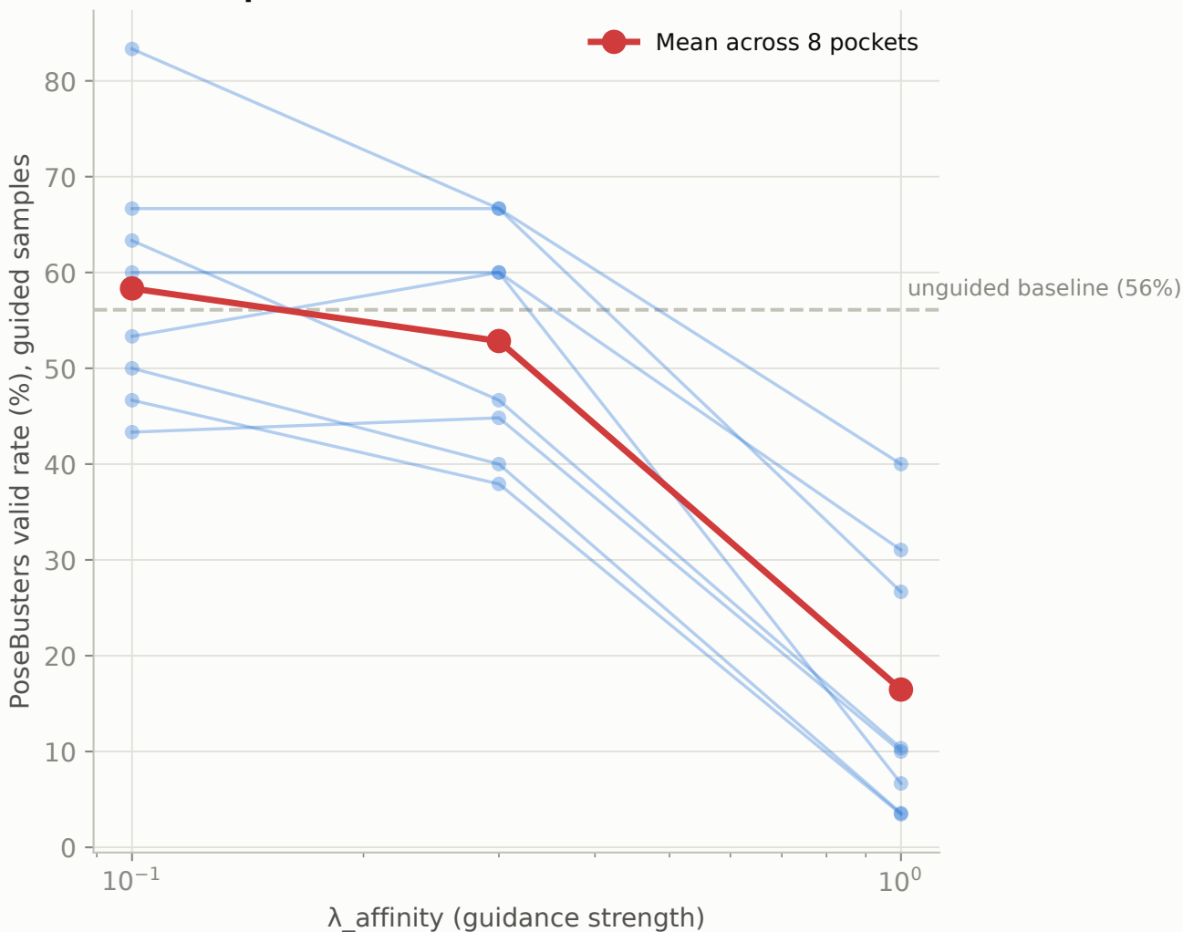
Track A: PoseBusters validity collapses with guidance strength (100% of pockets affected at \lambda=1.0 )
