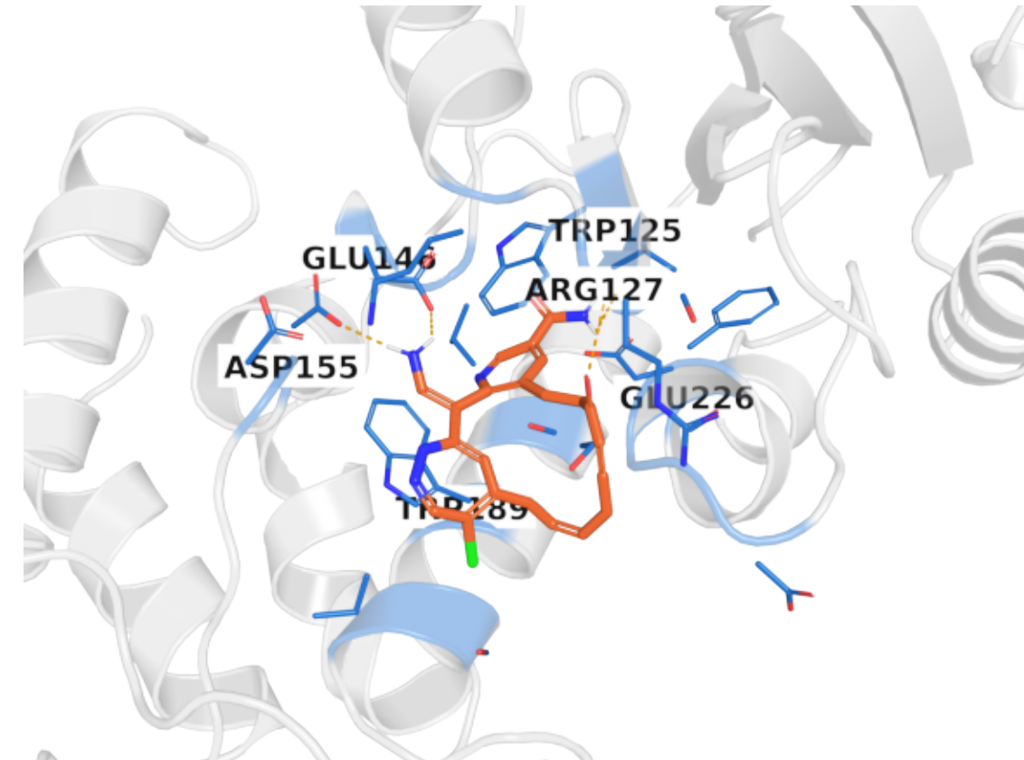
C. CD38_HUMAN (Vina Dock = -13.01)
