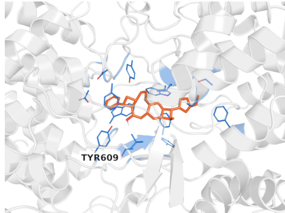
A. SQHC_ALIAD (Vina Dock = -15.79)
