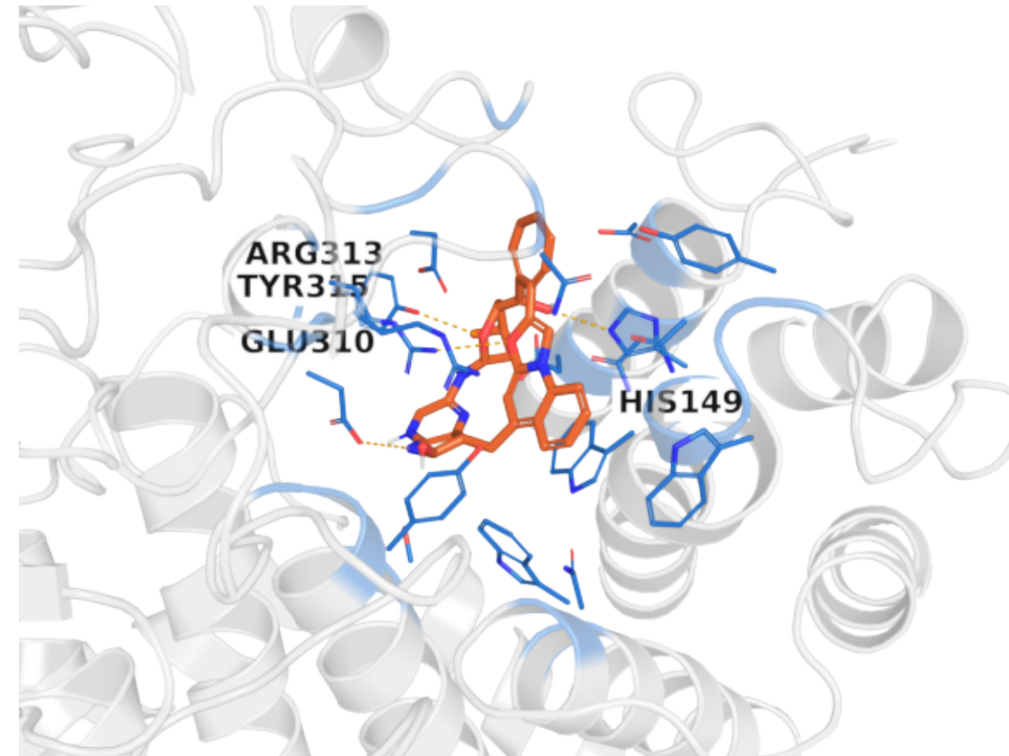
B. XANLY_BACGL (Vina Dock = -14.09)
